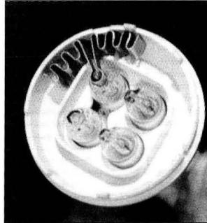
A rippled copper strip attached to the glass tubulation in a CFL rapidly conducts heat away from the lamp.
