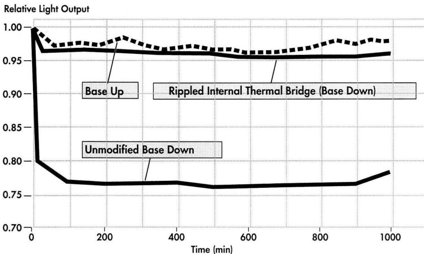
The base-up alternative produces almost 100% of the rated light output. The light output from the base-down CFL decreases by almost 25% after a few minutes of operation. However, by adding a thermal bridge (see opposite photos), the performance of the base-down CFL improves dramatically.
