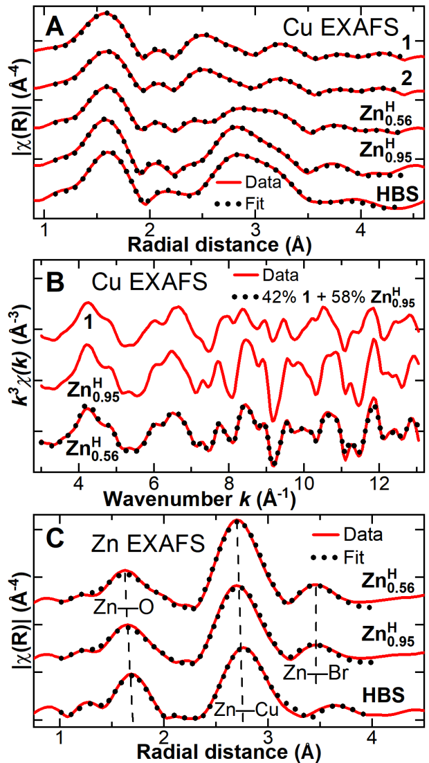
FIG. 2. A) Real-space Cu K-edge EXAFS data and fits of barlowite 1, barlowite 2, \text{Zn}_{0.56}^{\text{H}} , \text{Zn}_{0.95}^{\text{H}} , and herbertsmithite (HBS) showing the magnitude of the Fourier-transformed EXAFS ( \chi(R) ) measured at T = 10 K. B) Linear component fit of normalized \text{Zn}_{0.56}^{\text{H}} Cu EXAFS data of barlowite 1 and \text{Zn}_{0.95}^{\text{H}} . C) Real-space Zn K-edge EXAFS data and fits to \text{Zn}_{0.56}^{\text{H}} , \text{Zn}_{0.95}^{\text{H}} , and herbertsmithite (HBS) measured at T = 10 K. The three paths for Zn-substituted barlowite are shown as dashed lines. Vertical offsets have been applied to separate the spectra.
