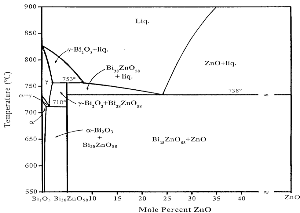
Figure 5.16. Phase diagram of the \text{Bi}_2\text{O}_3 and \text{ZnO} . 43
