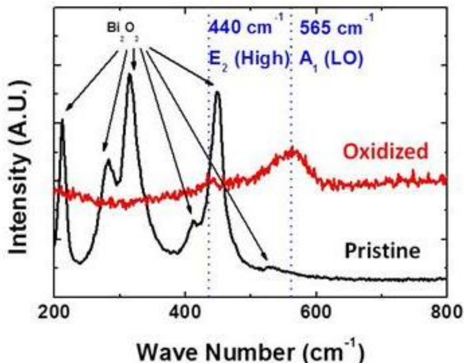
Figure 5.8. Raman spectra of the \text{Bi}_2\text{O}_3 electrode at pristine and oxidized (first discharged). The pristine sample is the \text{Bi}_2\text{O}_3 electrode after curing. The soaked sample is the \text{Bi}_2\text{O}_3 electrode after soaking in the electrolyte. The oxidized sample is the \text{Bi}_2\text{O}_3 electrode after first electrochemical oxidation or discharge.
