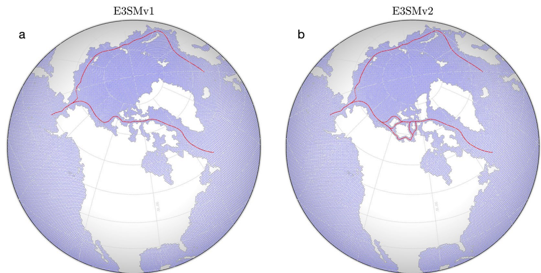
Figure 1. Comparison of the (a) old and (b) new standard resolution Energy's Energy Exascale Earth System Model (E3SM) unstructured marine mesh, highlighting improved geographic acuity in E3SMv2 including Arctic coastal shipping channels fitting standard routes published by the Arctic Council (2009) (red).
