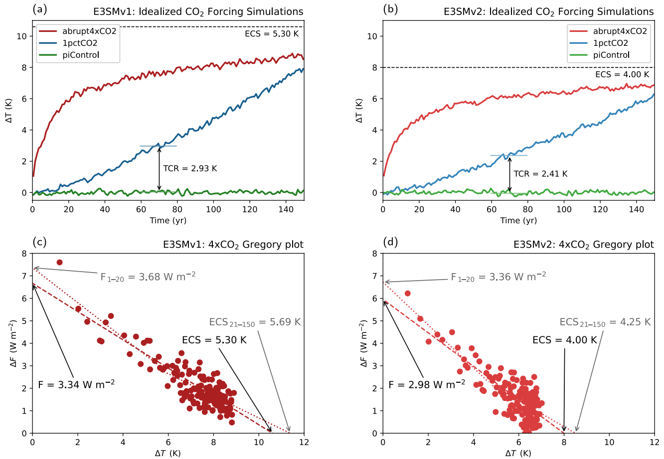
Figure 5. (a–b) Time evolution of annual global mean surface air temperature anomalies for the idealized CO_2 forcing simulations abrupt-4xCO2 (red), 1pctCO2 (blue), and the control simulation ( piControl ; green) for E3SMv1 and E3SMv2. The transient climate response (TCR) is computed as a 20 yr average around time of CO_2 doubling (year 70). (c–d) Gregory regression to estimate effective climate sensitivity (ECS) and effective 2xCO_2 radiative forcing ( F ) using the full 150 yr as well as the first 20 yr for the forcing ( F_{1-20} ) and the last 130 yr for the effective climate sensitivity ( ECS_{21-150} ).
