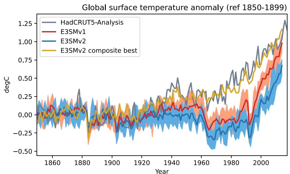
Figure 23. Time evolution of annual global mean surface temperature anomalies (with respect to 1850–1899). Comparison between observations from HadCRUT5-Analysis (gray), E3SMv1 ensemble mean (red) and range (orange) and E3SMv2 ensemble mean (dark blue) and range (light blue). Also shown (gold) is a best fit estimate obtained by scaling E3SMv2 GHG and aerosol as discussed in Section 5.
