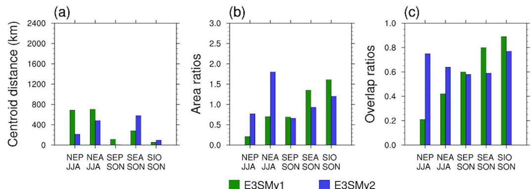
Figure 12. Centroid distances, area ratios, and overlap ratios of the LCC45+ decks in June–August (JJA) for the two Northern Hemisphere regions and in September–November (SON) for the Southern Hemisphere regions.
