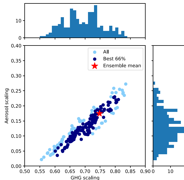
Figure B3. Scatter and distributions of optimal solutions \alpha_{\text{GHG}} and \alpha_{\text{aer}} for the loss function in Equation B1 using all 216 combinations of individual ensemble members or ensemble mean. Dark blue dots represent the best 66% solutions. Red star is the solution with ensemble mean for every term.
