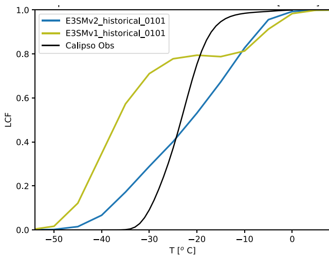
Figure 10. Diagnosed liquid cloud fraction (LCF) based on the monthly model output in the 30^{\circ} – 80^{\circ}S latitude band from (blue line) the E3SMv2 historical coupled simulation (1985–2014), (olive line) the E3SMv1 historical coupled simulations (1985–2014), and (black line) observations from Y. Hu et al. (2010).
