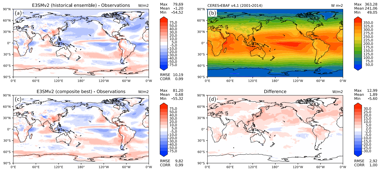
Figure 28. Net TOA SW radiation: observations (CERES-EBAF 4.1; b), model error for E3SMv2 (a), composite best configuration from Figure B1 in Appendix B (c), and difference between E3SMv2 and composite best configuration (d). Model and observations averaged over 2001–2014.
