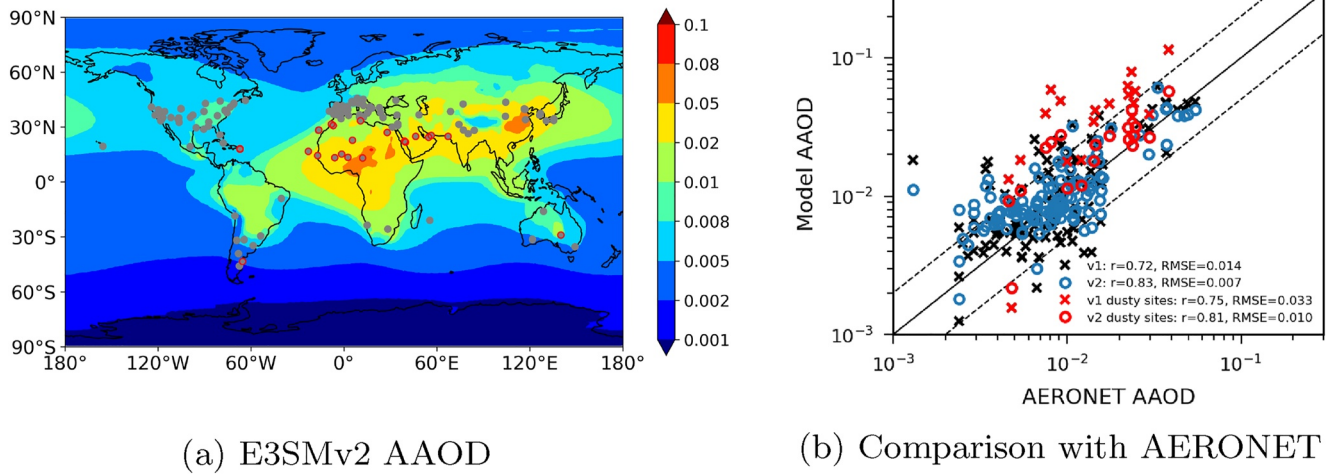
Figure 22. (a) Annual mean aerosol absorption optical depth (AAOD) at 550 nm in E3SMv2 for the time period 2000–2014. The gray dots overlaid on top denote the locations of 139 AERONET stations, of which those circled in red denote the 19 dusty sites. (b) Comparison of the E3SMv2 AAOD with the observations derived from AERONET between 2006 and 2015 (Holben et al., 1998). r is the calculated correlation coefficient, and RMSE is the root-mean-square error.
