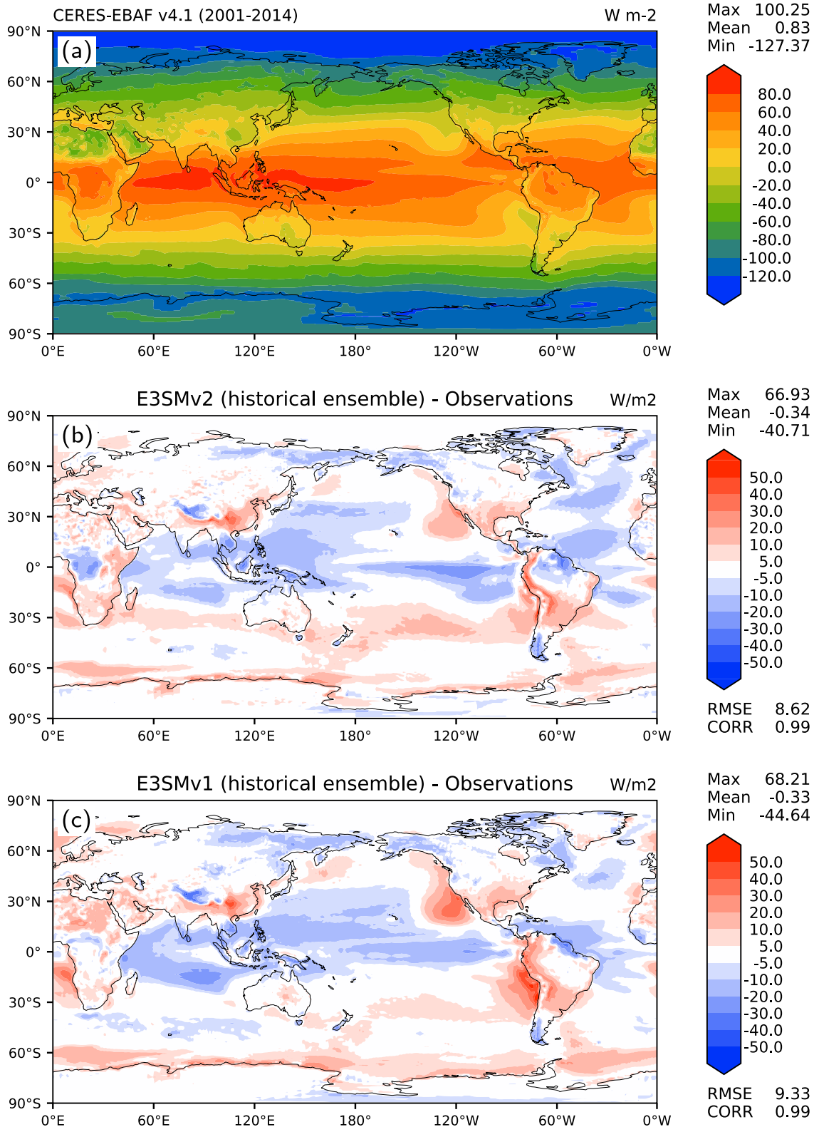
Figure 8. Annual net top-of-atmosphere (TOA) radiative flux ( W m^{-2} ): (a) CERES-EBAF Ed4.1 observational estimate (2001–2014), (b) model bias from the 5-member ensemble of E3SMv2 historical coupled simulations (2001–2014), and (c) model bias from the 5-member ensemble of E3SMv1 historical coupled simulations (2001–2014). RMSE, root-mean-square error; CORR, linear correlation coefficient between observation and model.
