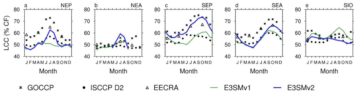
Figure 11. The mean low cloud cover (LCC) for each of the LCC45+ cloud decks (see text for definitions) for the 30° latitude by 35° longitude boxes over the Northeast Pacific (NEP), Northeast Atlantic (NEA), Southeast Pacific (SEP), Southeast Atlantic (SEA), and the Southern Indian Ocean (SIO).
