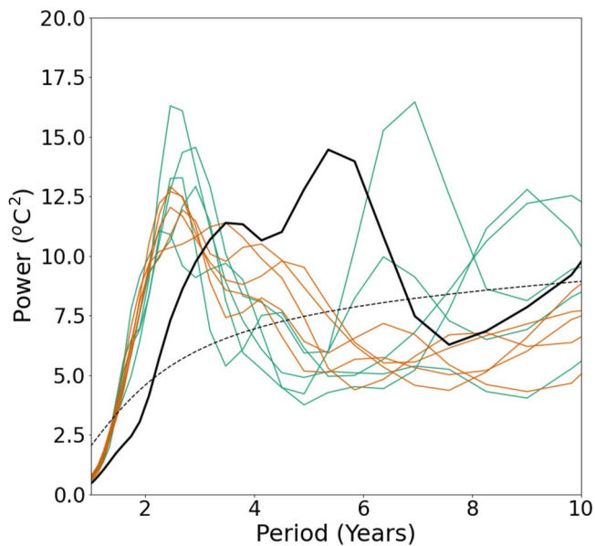
Figure 16. El Niño–Southern Oscillation (ENSO; Nino3.4) variability of the pre-industrial (PI) control simulation and historical ensemble. The Morlet wavelet of degree 6 is used (e.g., Torrence & Compo, 1998). The PI control (green lines) has been divided into five 100 yr sections; each Historical ensemble member is shown as an orange line. ERSSTv4 data (W. Liu et al., 2015) is shown as the thick black line. The 90% confidence interval is shown as the dashed black line.
