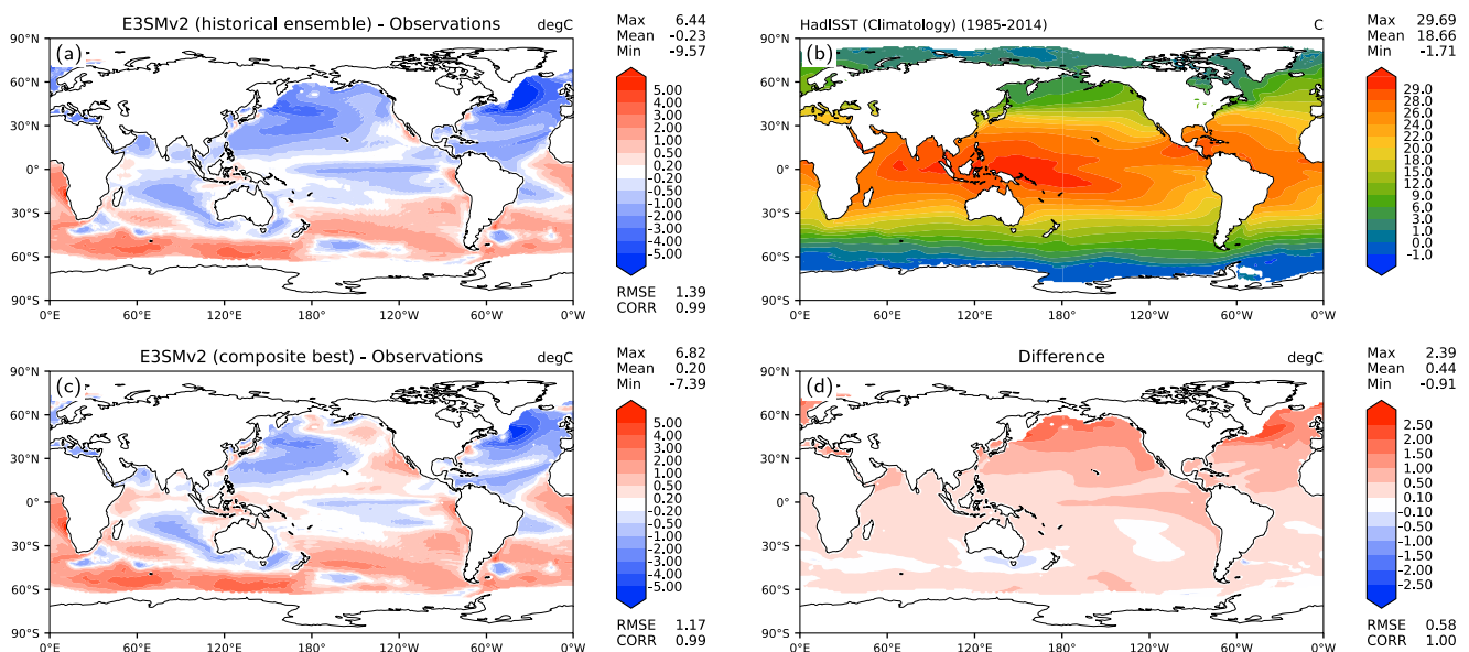
Figure 29. Same as Figure 28 but for SST. Sea ice covered regions are excluded from the averaging. Model and observations averaged over 1985–2014.
