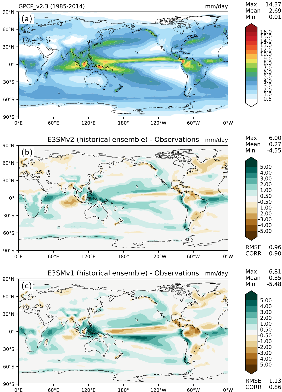
Figure 13. Annual precipitation rate (mm/day): (a) Global Precipitation Climatology Project v2.3 observational estimate (1985–2014), (b) model bias from the 5-member ensemble of E3SMv2 historical coupled simulations (1985–2014), and (c) model bias from the 5-member ensemble of E3SMv1 historical coupled simulations (1985–2014). RMSE, root-mean-square error. CORR, linear correlation coefficient between observation and model.
