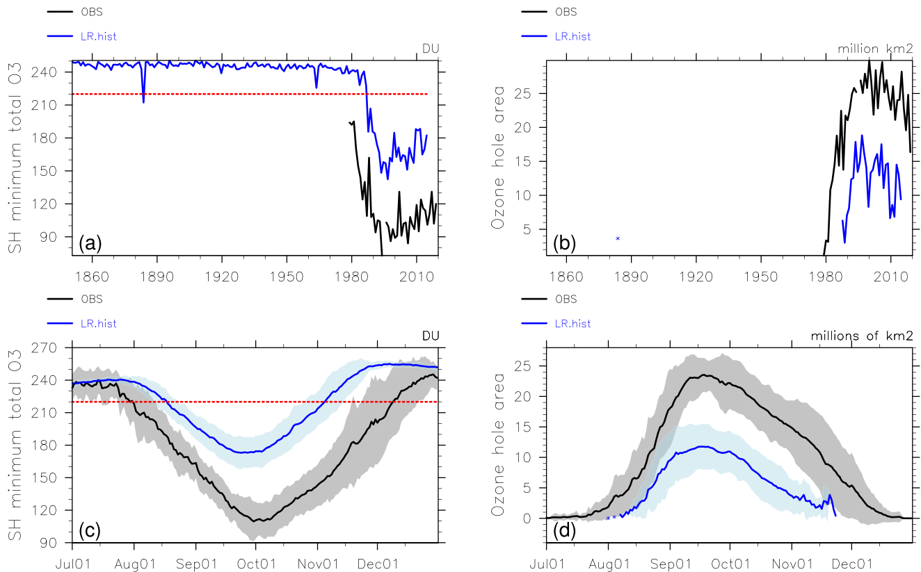
Figure 20. Ozone hole results as shown in the historical time series (top) and daily mean climatology and variance (bottom) of the SH minimum total column ozone (left, unit: DU) and the SH maximum ozone hole area (right, area with total ozone <220 DU, unit: million km 2 ) based on the daily data from 1 July to 31 December. In the bottom panels, the lines indicate the multiyear (1990–2014) average (observations in black and models in blue), and shading covers \pm 1 standard deviation.
