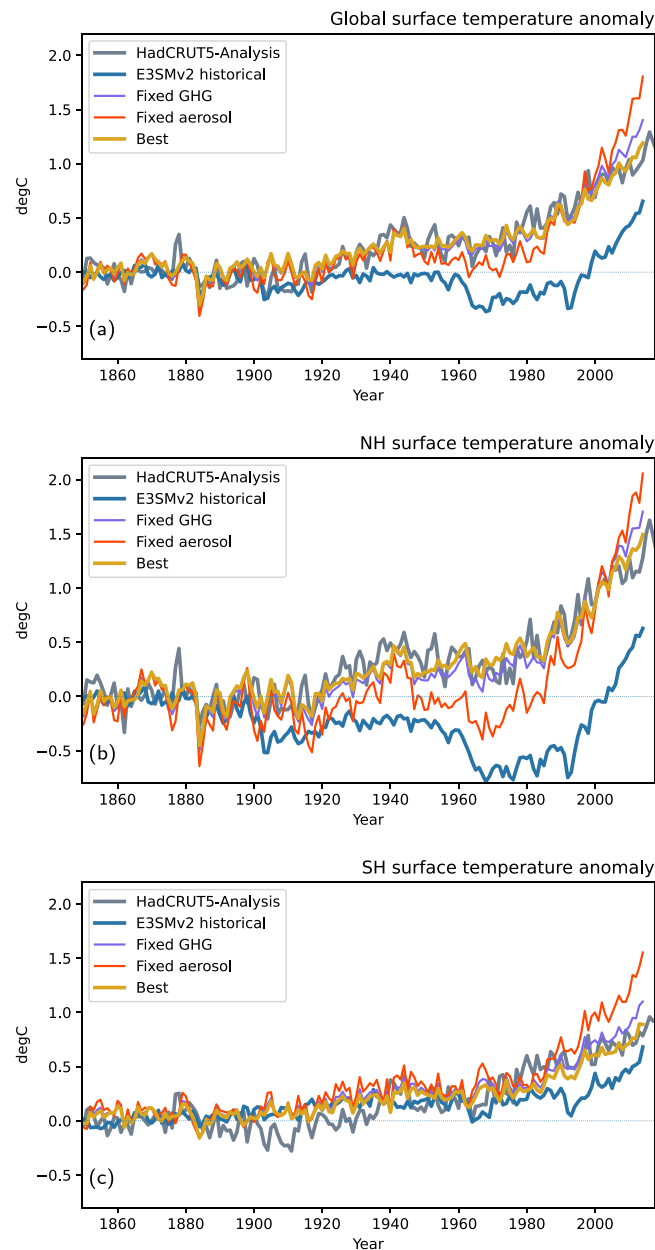
Figure B2. Surface temperature anomalies (with respect to 1850–1899) for (a) global, (b) Northern Hemisphere, and (c) Southern Hemisphere. Lines shown include observations (HadCRUT5-Analysis, gray), E3SMv2 (blue), and composite configurations from Figure B1 (red, purple, red, gold).
