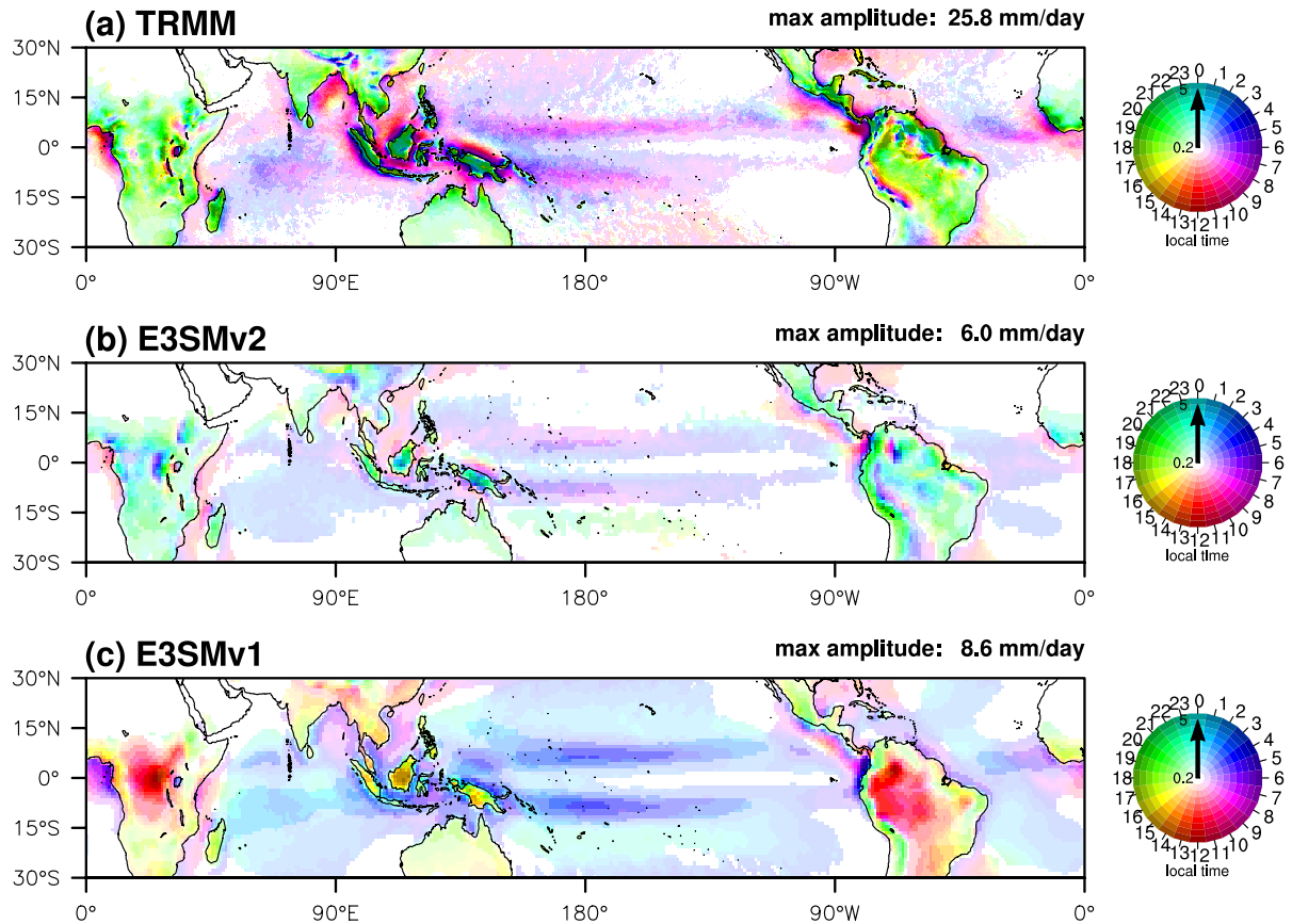
Figure 14. Annual mean time phase (color) and amplitude (color density) of the first diurnal harmonic of 3-hourly total precipitation (mm/day) from (a) TRMM (1998–2013), and historical simulations (1985–2014) of (b) E3SMv2 and (c) E3SMv1. Note that the diurnal properties are computed at 0.25^\circ resolution for TRMM and 1^\circ resolution for the models. Remapping the TRMM data to 1^\circ resolution does not lead to noticeable changes in the diurnal phases, though the amplitudes would be reduced somewhat due to spatial averaging (maximum amplitude over the tropics reduced to 18.9 mm/day from 25.8 mm/day). To ease comparison, the same amplitude upper bound is used for the plots, though the maximum amplitudes, as printed above each panel, are different. Amplitudes exceeding the upper bound are shown in the highest color density. Areas with diurnal amplitude less than 0.2 mm/day are left blank.
