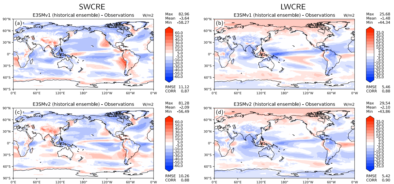
Figure 9. Annual top-of-atmosphere shortwave and longwave cloud radiative effect model biases (historical ensemble, 2001–2014) compared to CERES-EBAF Ed4.1 observational estimate (2001–2014) ( W m^{-2} ): (a) SWCRE E3SMv1, (b) LWCRE E3SMv1, (c) SWCRE E3SMv2, (d) LWCRE E3SMv2. RMSE, root-mean-square error. CORR, linear correlation coefficient between observation and model.
