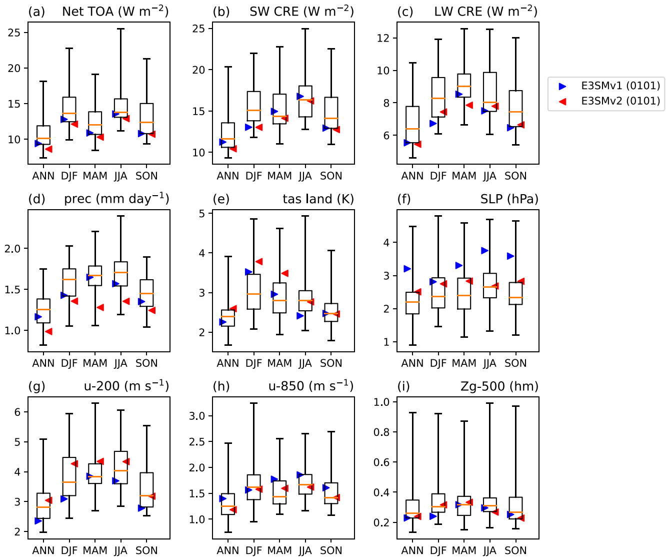
Figure 7. Comparison of RMSEs (1985–2014) of an ensemble of 52 CMIP6 models (first historical members r11p1f1) with the first historical members of E3SMv1 (blue triangles) and E3SMv2 (red triangles). Box and whiskers show 25th, median, 75th percentile, minimum, and maximum RMSE for the CMIP6 ensemble. Spatial RMSE against observations are computed for annual and seasonal averages with the E3SM Diagnostics package (C. Zhang et al., 2022). Fields shown include TOA net radiation (a), TOA SW and LW cloud radiative effects (b, c), precipitation (d), surface air temperature over land (e), sea-level pressure (f), 200 and 850 hPa zonal wind (g, h), and 500 hPa geopotential height (i). TOA, top-of-atmosphere; SW, shortwave; CRE, cloud radiative effects; LW, longwave; DJF, December–February; MAM, March–April; JJA, June–August; SON, September–November; RMSE, root-mean-square error. The mean climatology of the reference observational and reanalysis data sets are derived from: CERES-EBAF Ed4.1 (Loeb et al., 2018; 2001–2014) for (a–c), GPCP2.3 (Adler et al., 2018; 1985–2014) for (d) and ERA5 (Hersbach et al., 2020; 1985–2014) for (e–h). Due to data availability, not all models are included for every variable. Complete data is available in Table S1.
