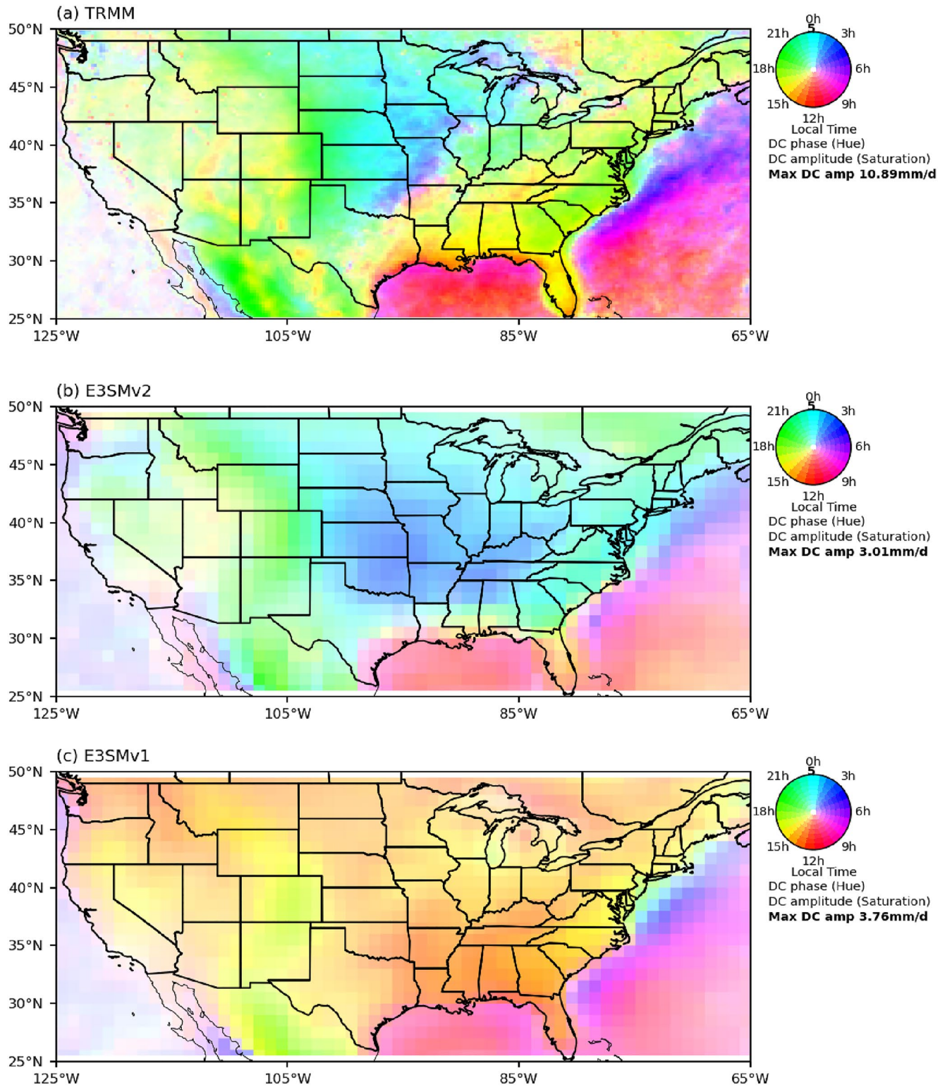
Figure 15. Same as Figure 14 except for the contiguous United States in June–July–August season.
