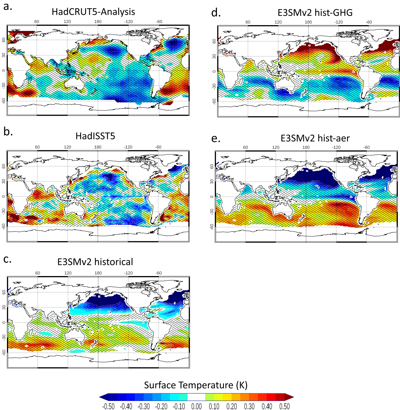
Figure 24. Difference in SST between 1980–2014 and 1870–1904 relative to the tropical mean change between the two periods for (a) HadCRUT5 data, (b) HadISST data, (c) E3SMv2 historical ensemble, (d) E3SMv2 hist-GHG ensemble, and (e) hist-aer ensemble. Hatched areas indicate regions where the difference is statistically significant at the 95% confidence level based on a two-tailed Student's t test.
