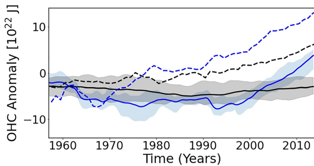
Figure 25. Ocean heat content (OHC) from the E3SMv2 historical ensemble. Blue shows the 0–700 m integrated OHC, and black shows the 700–2,000 m heat content. The solid lines are the ensemble average and shading shows the ensemble spread. The dashed lines are pentad-averaged OHC derived from the World Ocean Atlas 2009 (Levitus et al., 2012).
