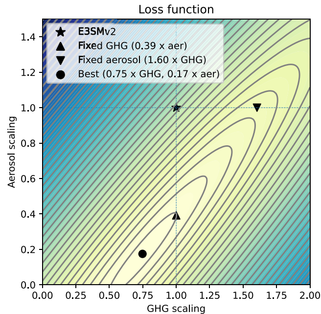
Figure B1. Loss function from Equation B1. Star represents E3SMv2, circle global minimum, and triangles local minima by minimizing along a single dimension.
