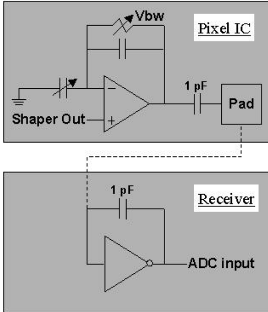
Fig. 6. “Active termination” output stage.
