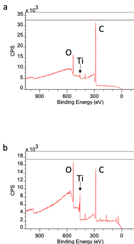
Figure 8. (a) XPS survey spectra of acid-etched Ti microfiber scaffold. The intensity of carbon is prominent. (b) XPS survey spectra of the UV-treated acid-etched Ti microfiber scaffold. The intensities of oxygen and Ti is increased. O, oxygen; Ti, titanium; C, carbon.
