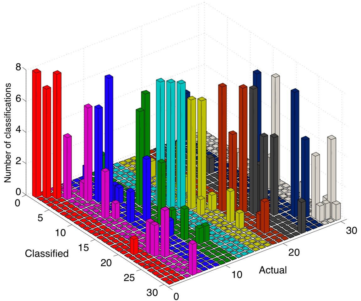
Figure 5.18: Confusion matrix for classifications using 5 multiple-frame Bark cepstrum coefficients.
