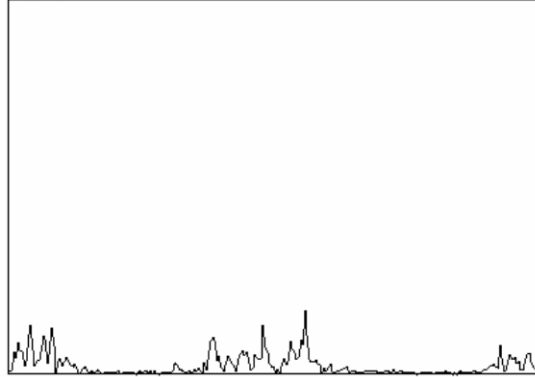
Figure 3.2: A tambourine spectrum with flatness value of 0.42.
