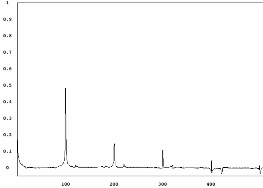
Figure 3.5: A cepstral quefrency peak resulting from a 440 Hz sawtooth wave.
