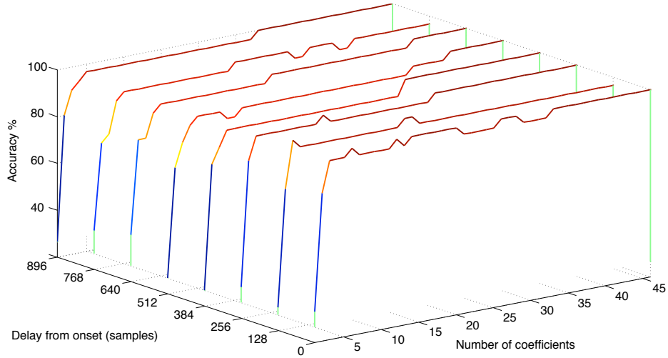
Figure 5.4: CR vs. OD vs. accuracy for BFCCs.
