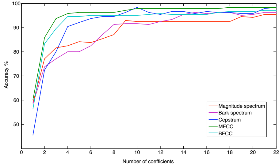
Figure 5.6: Accuracy vs. coefficients for all high level features using multiple-frame analysis.
