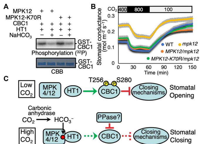
Fig. 7. The kinase inactive MPK12 isoform is sufficient for stomatal CO 2 sensing. (A) In vitro phosphorylation assays were performed after CBC1, HT1 and MPK12, or the MPK12-K70R kinase inactive isoform proteins were incubated with or without NaHCO 3 or NaCl (–) controls. (B) Stomatal conductances were analyzed in leaves of intact Arabidopsis plants [Col-0 (WT), mpk12 , pG1:MPK12-GFP/mpk12 and pG1:MPK12(K70R)-GFP/mpk12 ]. CO 2 concentration changes were applied as indicated on top (parts per million). n = 6 experiments. Error bars show ± SEM. (C) Model of plant stomatal CO 2 sensor and signaling (see main text). An unknown protein phosphatase (PPase) is assumed to inhibit CBC1 at high CO 2 for activation of stomatal closing mechanisms.
