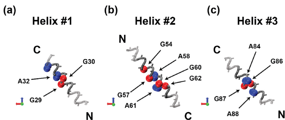
Fig. 7. Glycine-Alanine Packing Surfaces. (a) – (c) Model helices based on the experimentally determined tilt and rotation angles for each helix of Rv1861. Glycine C_\alpha residues are shown as red spheres, alanine C_\alpha/C_\beta residues as blue spheres and all other residues represented as C_\alpha/C_\beta bonds. Translucent sections of helix reside outside the well-defined core region for each helix.
