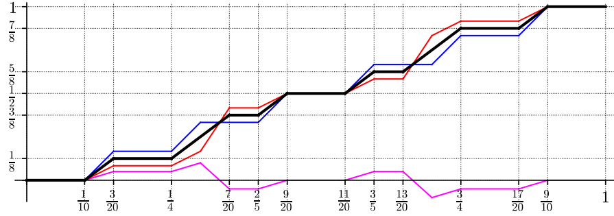
Fig. 4: Continuous 2-slope maximal non-extreme cDFF w_{2slope\_3covered\_nonextreme} (in black), an effective perturbation function \tilde{\pi} (magenta), and functions \phi^\pm = \phi \pm \epsilon\tilde{\phi} (blue and red).
