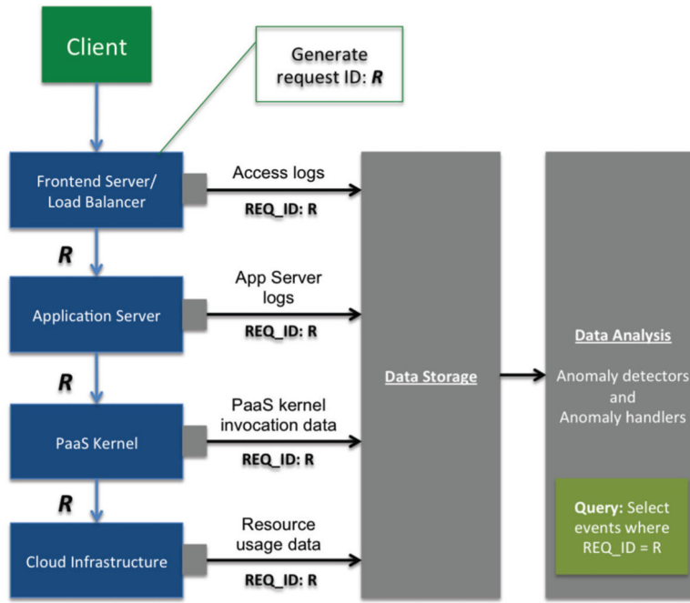
Fig. 1. Roots APM architecture.
