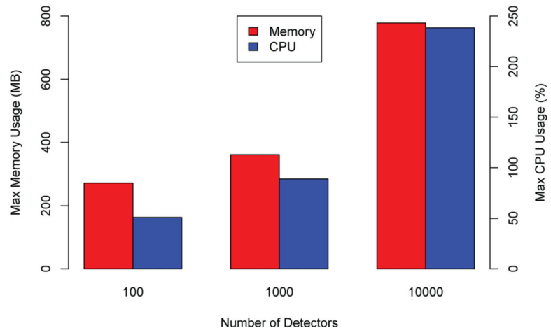
Fig. 12. Resource utilization of a Roots pod.
