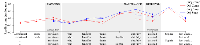
Figure 3: Residualized log reading times for Experiment 2
