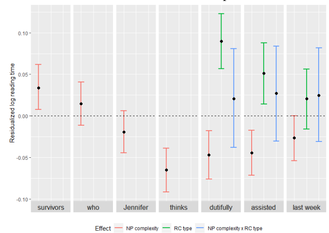
Figure 4: Credible intervals for Experiment 2
