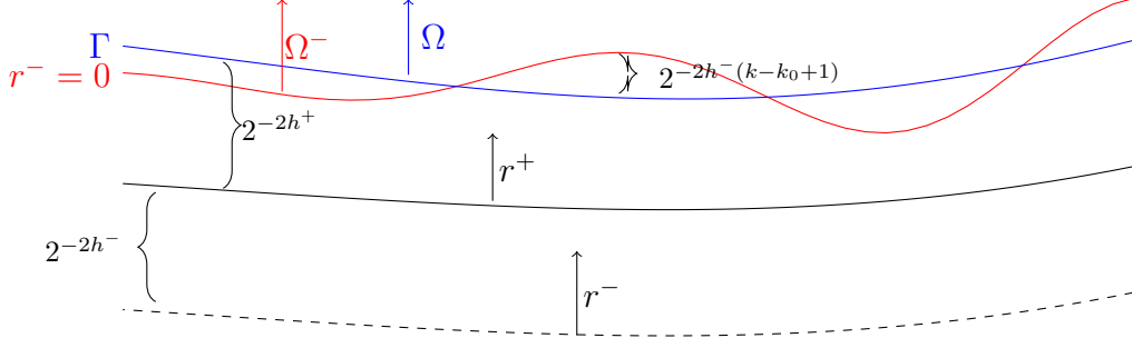
FIGURE 3. Domains associated with the regularization scheme.
