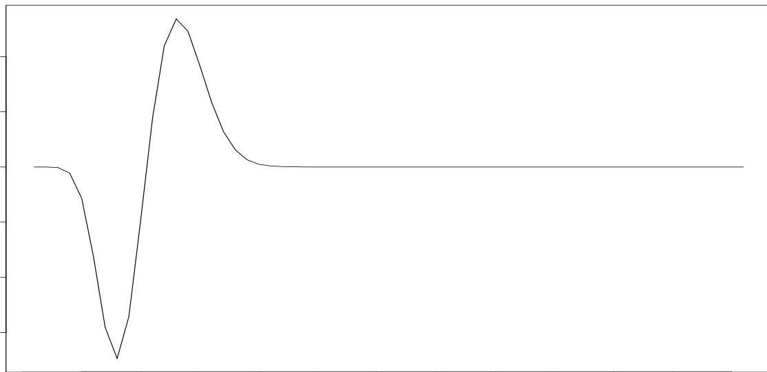
Figure 0.6: P(N = i | \hat{\lambda}_{Poisson} = x) - P(N = i | \hat{\lambda}_{BAYES} = x) vs. i
