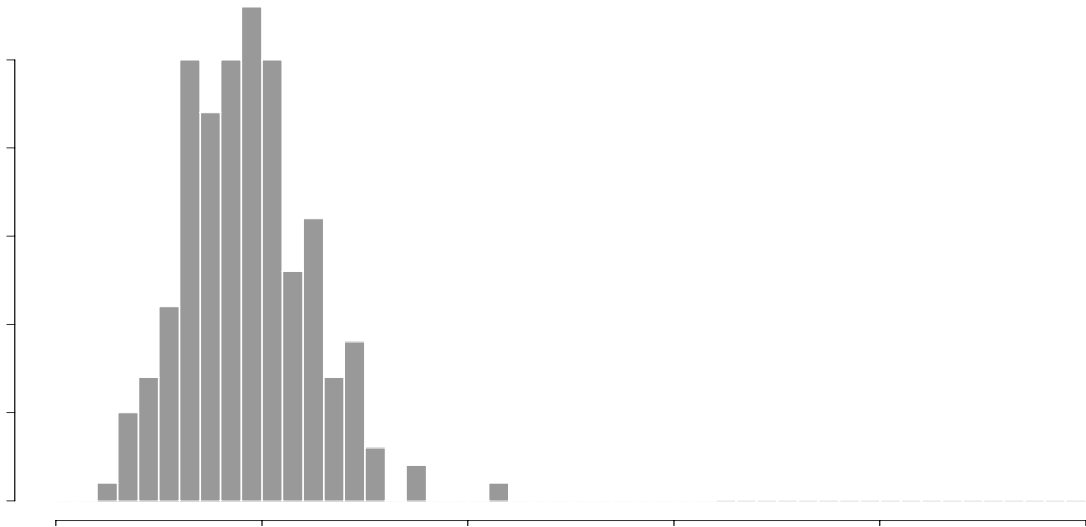
Figure 0.8: Histogram of R for 200 standard Poisson processes
