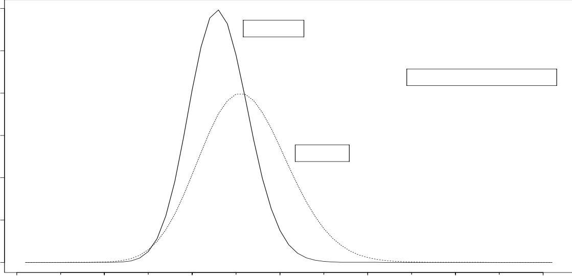
Figure 0.3: P(N = i | \hat{\lambda}_{BAYES} = x) and P(N = i) vs. i
