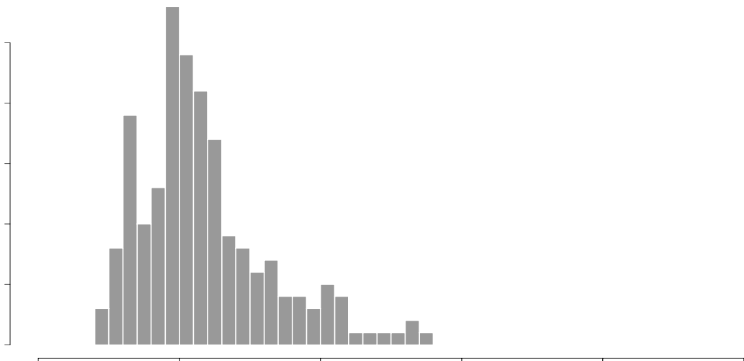
Figure 0.9: Histogram of R for 200 Gamma-transformed processes
