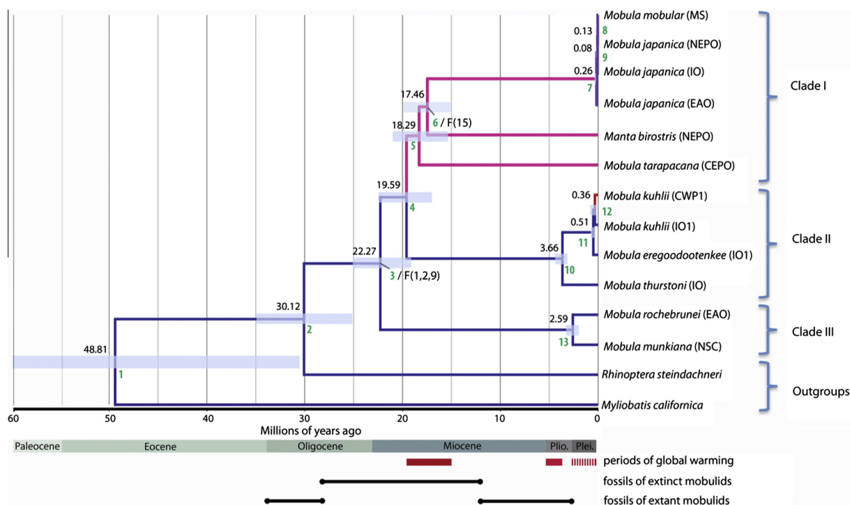
Fig. 4. Divergence time estimates based on analysis of the mitogenome BEAST data set. Point estimates of ages are given above each node and transparent blue horizontal bars denote age (95% highest posterior density). Branch colors show relative nucleotide substitution rates (blue is slow, purple intermediate, red fast). F(1, 2, 9) and F(15) denote fossil calibration points (numbers 1, 2, 9 and 15 refer to Supplementary Table S4). Green numbers on nodes are explained in the text. Red bars below the epoch bar denote periods of global warming and associated low upwelling intensities. Black lines below that denote timing of occurrence of extinct and extant mobulid species based on the fossil record (see Supplementary Table S4).
