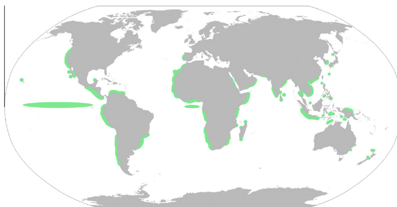
Fig. 6. Modern-day upwelling regions of the world, based on Alongi et al. (2012); Darbyshire (1967), Defant (1936), Fang et al. (2012), Furnestini (1959), Hasegawa et al. (2009), Ikema et al. (2013), Krishna (2011), Lafond (1954,1957), Lutjeharms and Machu (2000), Ma et al. (2013), Mazeika (1967), Rama Sastry and Myrland (1959), Roughan and Middleton (2002), Smith and Suthers (1999), Stommel and Wooster (1965), Swallow and Bruce (1966), Vinayachandran and Yamagata (1998), Warren et al. (1966), Wooster and Reid (1963), Wooster et al. (1967), Wyrteki (1961,1962, 1964, 1966) and Zaytsev et al. (2003).
