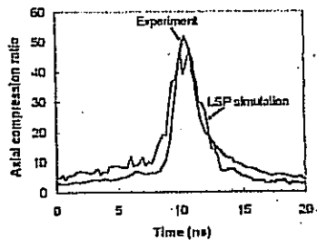
FIG. 12: Comparison of beam compression between experiment and LSP simulation for the 2-m long plasma column.
