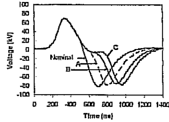
FIG. 3: Induction module voltage waveforms produced by varying the timing of the modulators.
