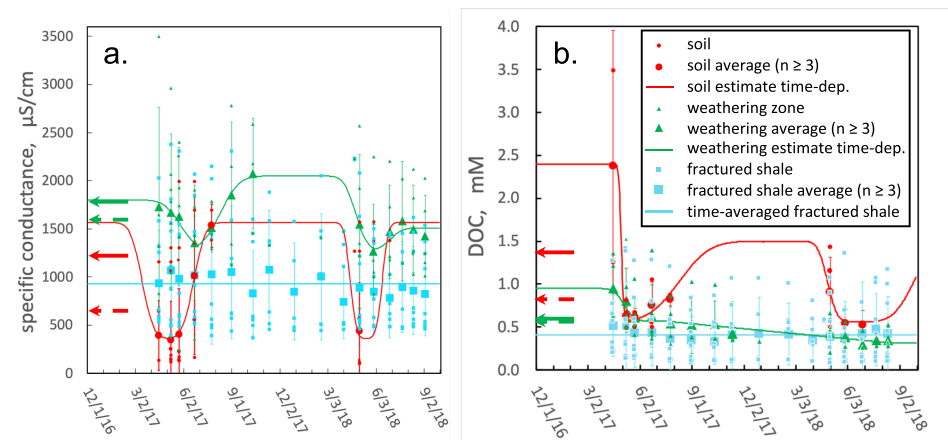
Figure 9. Time trends in pore water specific conductance (a) and DOC (b). The analyses of PLM1–3 pore waters are grouped into three zones; soil (to 1.00 m depth), weathering zone (1.00 to 3.60 m), and fractured shale (deeper than 3.60 m). Horizontal arrows along the vertical scales indicate average values of data (dashed) and curve-fit trends (solid) for the soil (red) and weathering zones (green), respectively.
