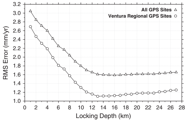
Figure 7. Plot of model fit to GPS (RMS error) for a range of locking depths. A 13 km locking depth minimizes misfit; however, locking depths greater than 12 km do not offer significantly worse fit to the data overall.
