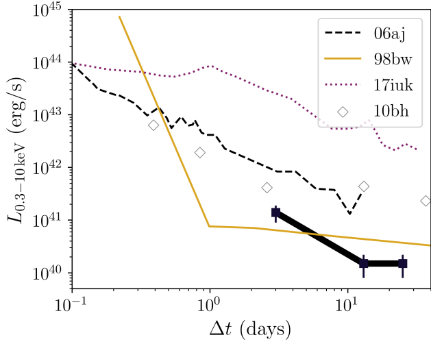
Figure 15. The 0.3–10 keV X-ray light curve of SN 2020bvc (black connected squares) compared to that of nearby Ic-BL SNe associated with LL-GRBs. Data on GRB-SNe taken from Campana et al. (2006), Corsi et al. (2017), and D’Elia et al. (2018).
