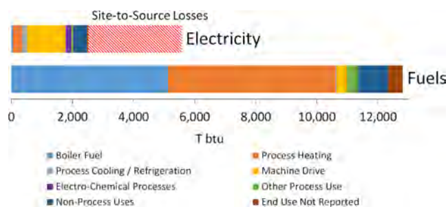
Fig. 12. Distribution of energy end-uses in the U.S. manufacturing sector in 2014. The top bar shows end uses of electricity (including site-to-source losses) and the bottom bar shows direct combustible fuel use [168].
