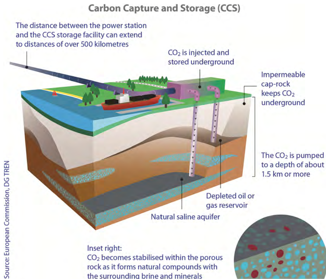
Fig. 11. An overview of underground carbon storage. Though this diagram indicates compressed CO 2 comes from a “power station,” it may also be produced by an industrial facility or a cluster of facilities. Image CC BY 4.0 European Commission (permission).
