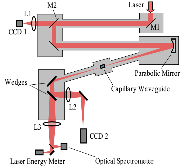
Figure 2: The experimental layout used for investigating laser beam propagation in a capillary waveguide. Laser pointing input to the capillary was measured by CCD 1.
