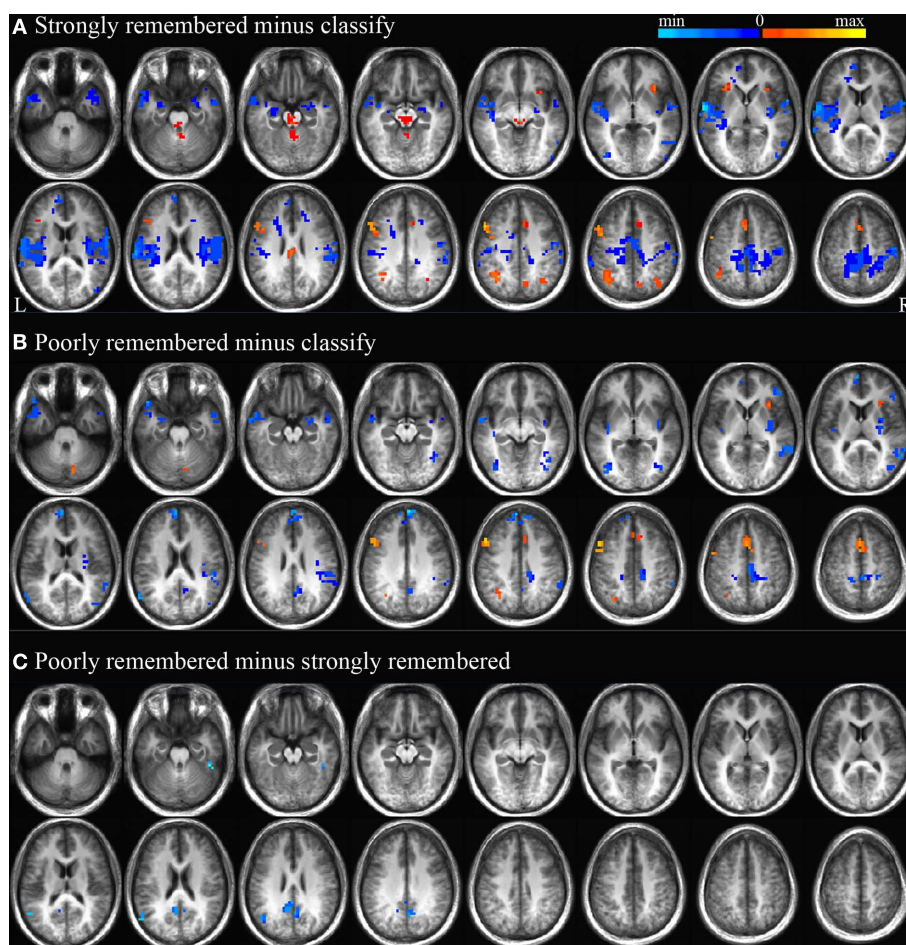
FIGURE 2 | Strongly remembered minus classify, poorly remembered minus classify, and poorly minus strongly remembered contrasts. Regions with significant BOLD signal differences ( p < 0.01 ) between strongly remembered and classify trials ( A ), poorly remembered and classify trials ( B ), and poorly and strongly remembered trials ( C ). Positive activity differences
