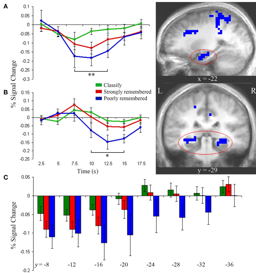
FIGURE 3 | Anterior and posterior hippocampal activity. (A) Left anterior hippocampus showed greater deactivation during strongly and poorly remembered relative to classify trials (right, p < 0.05 ). Impulse response curves (left) illustrate a graded pattern of deactivation from fixation baseline greatest for poorly remembered (blue), intermediate for strongly remembered (red), and minimal for classify (green) trials. **Indicates poorly remembered < classify, strongly remembered < classify, and poorly remembered < strongly remembered (paired t -tests, p < 0.01 ). (B) Bilateral posterior hippocampus was more active for strongly versus poorly
