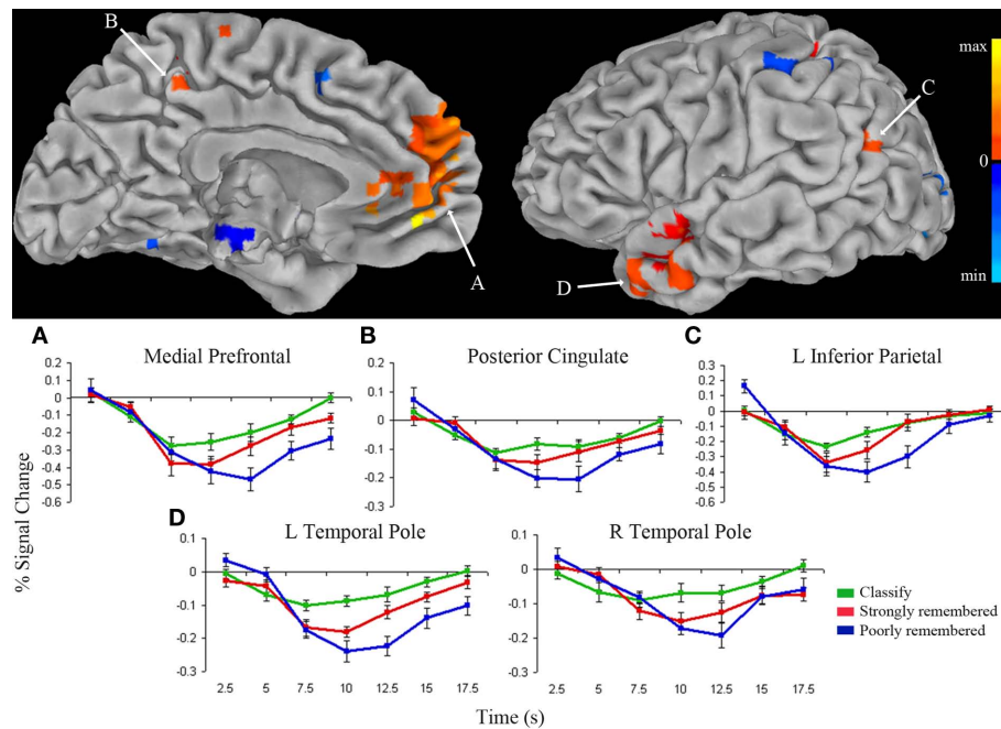
FIGURE 4 | Regions fitting the anterior hippocampus response model.
