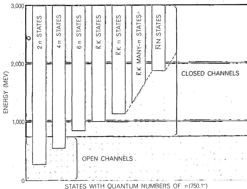
"COMMUNICATING CHANNELS" (vertical bars) are nuclear states that possess all the same quantum numbers as a particular particle, in this case \pi(750, 1^-) . Channels into which it has sufficient energy to decay are "open" channels. Channels for which it lacks sufficient energy are "closed." The threshold energy for gaining access to a communicating channel is the sum of the rest masses (in Mev) of the various particles constituting the channel.
