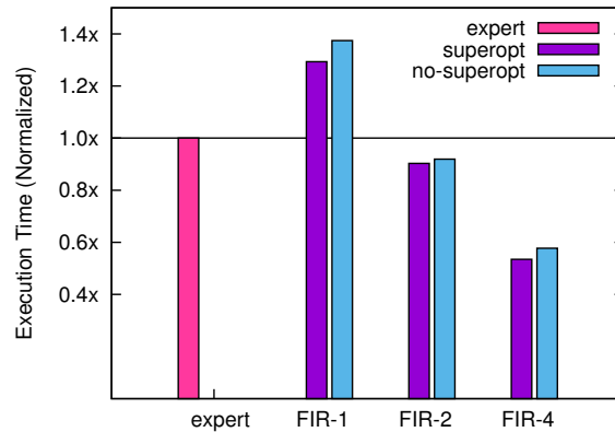
Figure 2.13: FIR benchmark
