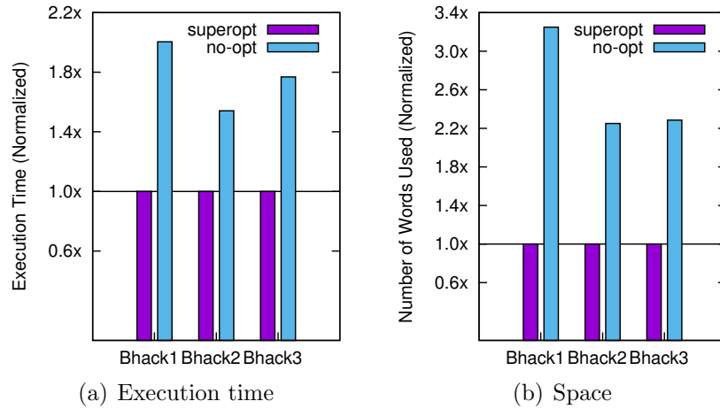
Figure 2.12: Bithack benchmarks
