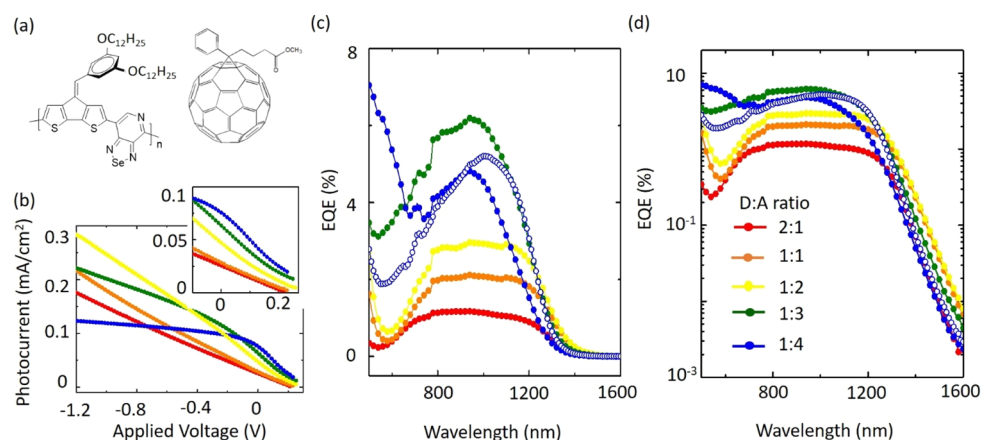
Figure 1. (a) Chemical structures of the polymer and fullerene derivative. (b) Photocurrent versus applied voltage under incident broad spectrum white light with the intensity of 4 mW/cm 2 . The light intensity was kept low to ensure all of the measurements were in the linear dynamic range of the devices. The inset zooms in near the built-in bias. The various colors indicate different donor to acceptor ratios. External quantum efficiency at zero applied bias versus incident wavelength, in (c) linear scale and (d) logarithmic scale. The BHJ film thickness for each D:A ratio is 180 nm for 2:1, 160 nm for 1:1, 190 nm for 1:2, 160 nm for 1:3, and 120 nm (blue solid symbols) and 200 nm (blue open symbols) for 1:4.
