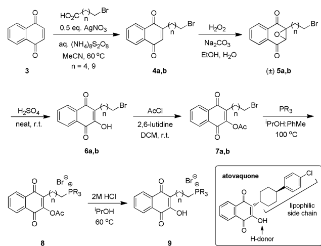
Scheme 1. Synthesis of 2-Hydroxy 1,4-Naphthoquinone Phosphonium Cation 9 (Table 1)
