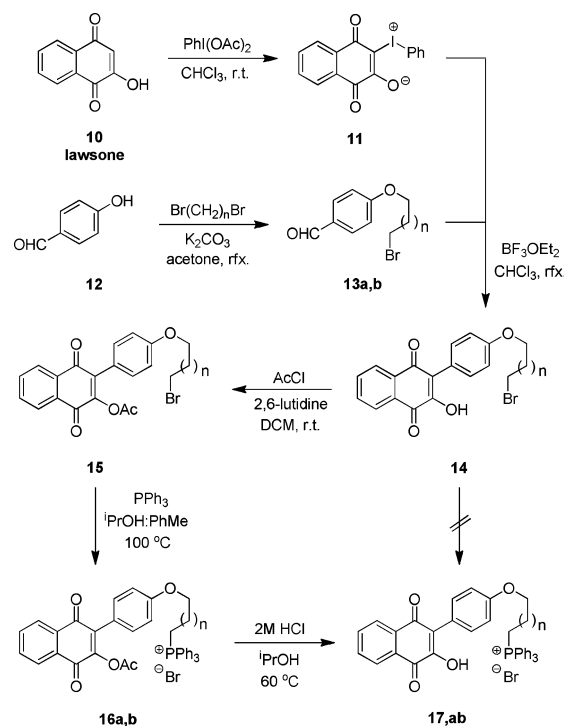
Scheme 2. Synthesis of 1,4-Naphthoquinone-Based Phosphonium Cations 16 and 17 (Table 1)
