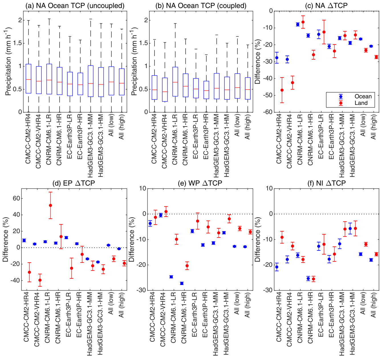
Figure 1. Boxplots of simulated tropical cyclone precipitation (TCP, mm h -1 ) from 1950–2014 in the (a) uncoupled and (b) coupled simulations by model, and their percentage difference ((coupled minus uncoupled)/ uncoupled), denoted as \Delta TCP over the (c) North Atlantic (NA), (d) eastern North Pacific (EP), (e) western North Pacific (WP), and (f) North Indian (NI) basins. While boxplots in (a and b) are based on TCP over ocean, blue and red error bars in (c–f) represent the \Delta TCP over ocean and land, respectively. The two rightmost boxes in (a and b) or blue/red bars in (c–f) refer to the ensemble of all low- and high-resolution model simulations, respectively. The 95% confidence interval in (c–f) is estimated from individually bootstrapping the uncoupled and coupled data 200 times and then calculating their percentage differences (in relative to the mean of uncoupled data) and associated bootstrap standard error.
