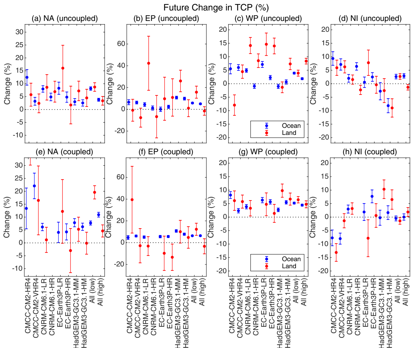
Figure 4. Percentage changes in 2015–2050 tropical cyclone precipitation (TCP) relative to 1950–2014 by model and basin in the (a–d) uncoupled and (e–h) coupled simulations. Blue and red error bars in each panel represent future changes in TCP over ocean and land, respectively. The basins include the North Atlantic (NA), eastern North Pacific (EP), western North Pacific (WP), and North Indian (NI). The two rightmost blue/red bars in each panel refer to the ensemble of all low- and high-resolution model simulations, respectively. The 95% confidence interval is estimated from individually bootstrapping the 2015–2050 and 1950–2014 data 200 times and then calculating their percentage differences (in relative to the mean of 1950–2014 data) and associated bootstrap standard error. The first red error bar in (e) extends beyond the figure because of its large uncertainty in future TCP change.
