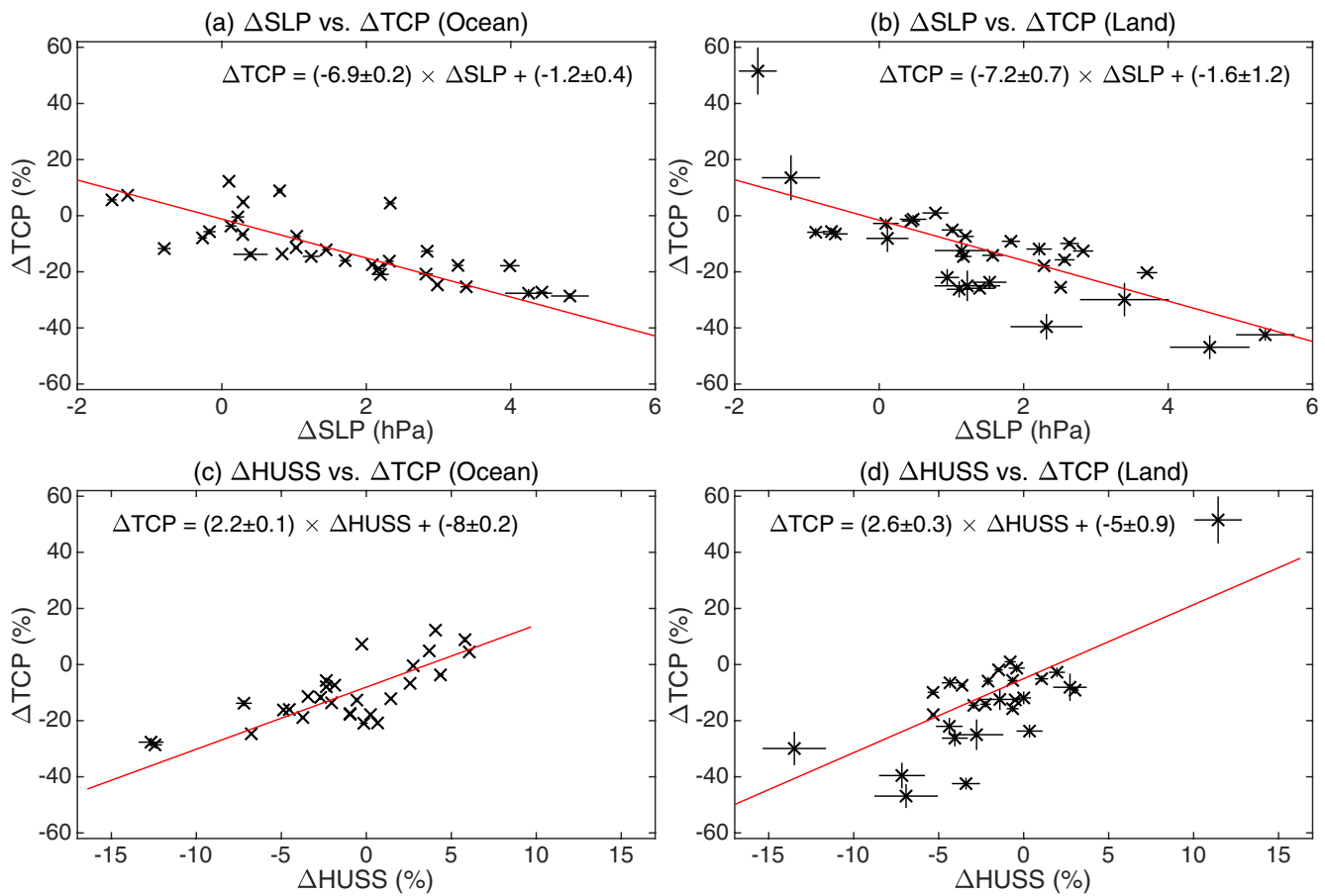
Figure 3. Differences in TC minimum sea level pressure ( \Delta SLP, hPa), near-surface specific humidity ( \Delta HUSS, %), and tropical cyclone precipitation ( \Delta TCP, %) between the coupled and uncoupled simulations over ocean (a and c) and land (b and d). Each point is derived from a unique combination of four ocean basins and seven/eight climate models ( \Delta HUSS data is not available in the CNRM-CM6.1-HR model), with the error bar representing its uncertainty range (mean \pm one standard deviation).
