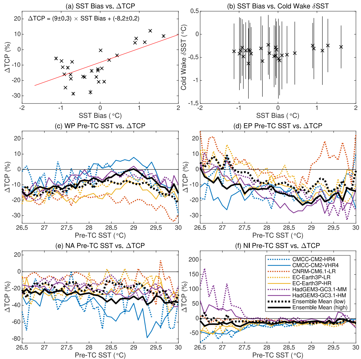
Figure 2. (a) Basin-scale sea surface temperature (SST) bias ( ^{\circ}\text{C} ) averaged over tropical oceans ( 5^{\circ} – 30^{\circ}\text{N} ) from the AOGCM and the percentage difference in ocean tropical cyclone (TC) precipitation ( \Delta\text{TCP} ) between the coupled and uncoupled simulations during the period from May–November 1950–2014. (b) Basin-scale SST bias and TC cold wake \delta\text{SST} ( ^{\circ}\text{C} ) in the coupled simulations. (c–f) Ocean-specific \Delta\text{TCP} with the same pre-TC SST (binned by 0.1^{\circ}\text{C} increment) in the coupled and uncoupled simulations. Each point in (a and b) is derived from a unique combination of four ocean basins and seven climate models (SST data is not available in the CNRM-CM6.1-HR model), with the error bar in y-axis representing its uncertainty range (mean \pm one standard deviation).
