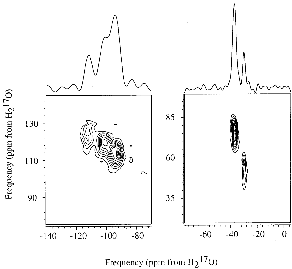
Figure 4.11: 11.7T 17 O 3QMAS of larnite (left) and forsterite (right).
