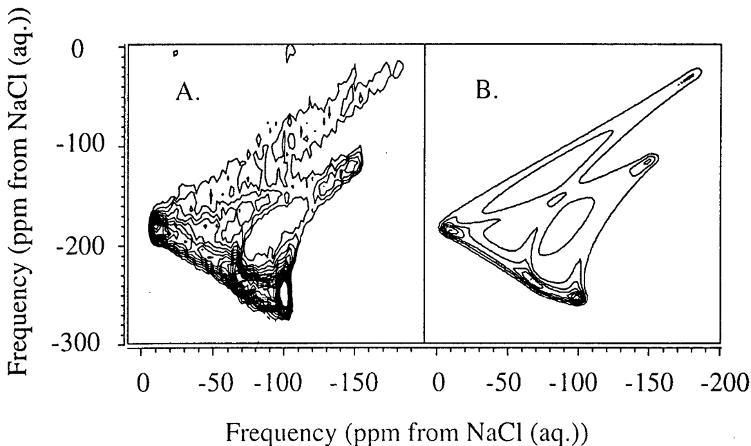
Figure 6.4: (A) Experimental and (B) simulated two-dimensional ^{23}\text{Na} SAS NMR spectra of \text{Na}_2\text{SO}_4 acquired at 4.2T with \theta_1 = 80^\circ, \theta_2 = 54.74^\circ . The simulated spectrum corresponds to C_Q = 2.6\text{MHz} , \eta_Q = 0.6 , and \delta_{iso} = 4\text{ppm} . No chemical shift anisotropy was included in the simulation. The horizontal dimension is the MAS dimension.
