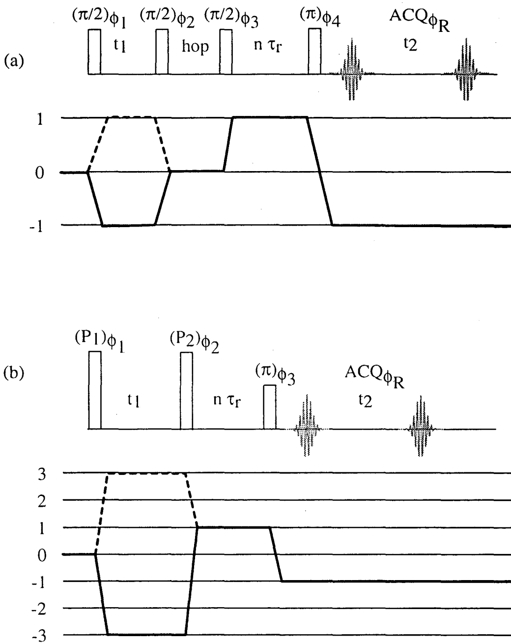
Figure 3.13: HyperSEDAS and HyperSEMCMAS experiments which acquire whole DAS or MCMAS echo in the t_2 dimension.
