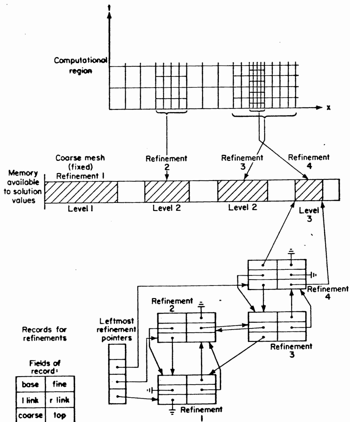
Figure 6.1 Data Structure: Tree and Vector of Deques
