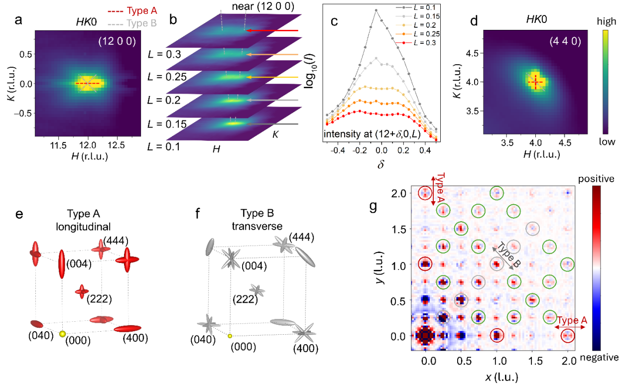
Figure 4. Near-Bragg diffuse scattering reveals collective displacements. a. Total scattering intensity near (12 0 0) in HK0 . Types A and B diffuse scattering are indicated by red and grey dashed lines, respectively. b. Reciprocal space views above (12 0 0) in L planes. c. Total scattering intensity along H paths as marked by arrows with corresponding colors in (b). d. Scattering intensity near (4 4 0) in HK0 . Summarized distribution of (e) Type A and (f) Type B diffuse scattering. g. 3D- \Delta PDF in xy0 at 300 K with a radius 0.2 r.l.u. Bragg punch. Red, grey, and green circles highlight displacements of predominantly longitudinal, transverse, and mixed origins, respectively.
