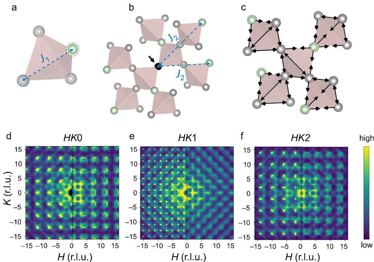
Figure 3. Simulations of chemical SROs and the local size effect. a-c. Modeled correlations among 16d sites. Representative metal pairs at (a) \langle \pm 1/4, \pm 1/4, 0 \rangle and at (b) \langle \pm 1/2, \pm 1/2, 0 \rangle with the characteristic chemical correlations, highlighted by blue dashed lines. Both energy terms J_1 and J_2 are positive, which lead to negative chemical correlations. Solid grey and smaller green spheres are In-occupied and Li-substituted sites, respectively. In b, a representative In-occupied reference site is highlighted in black. c. Size effect involving an elongated In-In distance and a shrunk In-Li distance with arrows pointing in the directions of displacements. Experimental observations (left) and MC-simulated diffuse scattering patterns (right) in (d) HK0 , (e) HK1 , (f) HK2 , intensity on a log scale.
