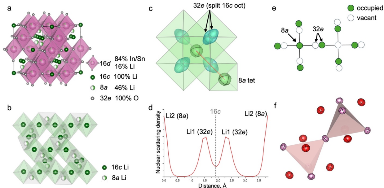
Figure 1. Average crystal structure derived from single-crystal diffraction. a. Crystal structure of LISO. b. Li network composed of face-sharing 8a and 16c sites. c. Fragment of the crystal structure refined from neutron data highlighting 50% Li ADP ellipsoids in 8a and 32e sites, with Li density isosurfaces in a translucent cyan color. d. Li nuclear density based on neutron diffraction along a Li2-Li1-Li1-Li2 path (red line in c ). e. Schematic of local Li site occupancy in 8a and 32e . f. Structural fragment highlighting the 95% In (purple) and O (red) ADP ellipsoids, based on single-crystal XRD.
