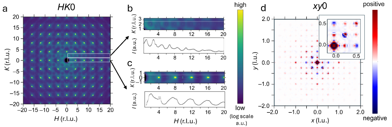
Figure 2. Symmetrized synchrotron X-ray total scattering and 3D-APDF. a. Total scattering in the HK0 plane at 300 K. b. Zoom-in view of the square-shaped diffuse scattering in HK0 and integrated intensity between K = 2.55 and 2.65 along H (white line). c. Enlarged view of the butterfly-shaped diffuse scattering in HK0 and integrated intensity between K = 0.55 and 0.65 along H (white line). d. 3D-APDF in the xy0 plane with a Bragg punch size of 0.2 r.l.u. at 300 K. Zoom-in view on the upper right corner.
