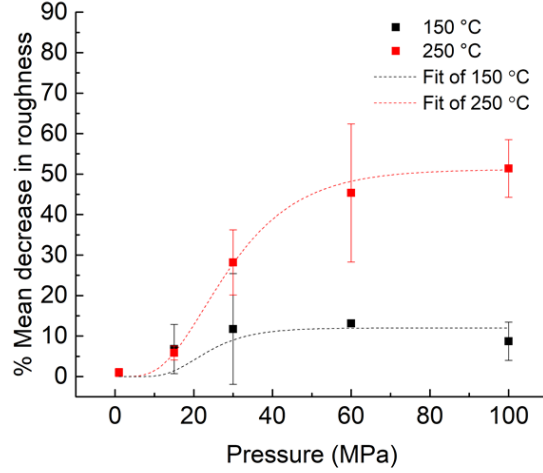
Fig 5. Percentage change in roughness after flattening at 150 and 250 °C.
