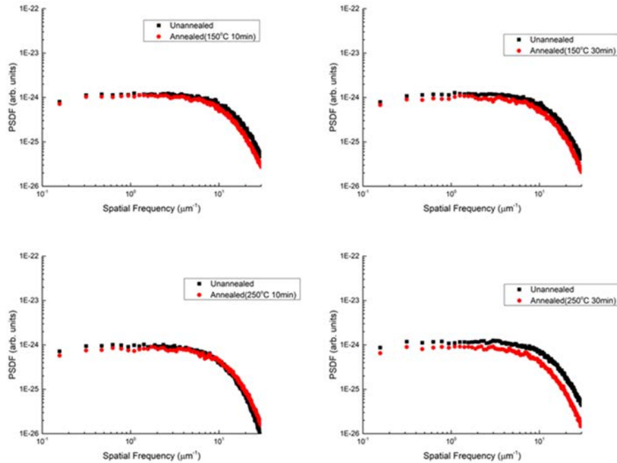
Fig 7: PSDF plots before and after annealing for 10 and 30
