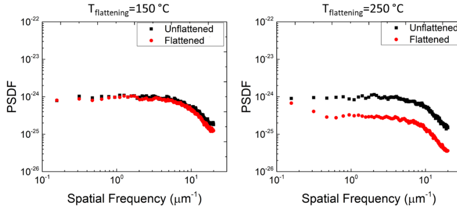
Fig 6. PSDF plots for T_{\text{flattening}} = 150 and 250 °C.
