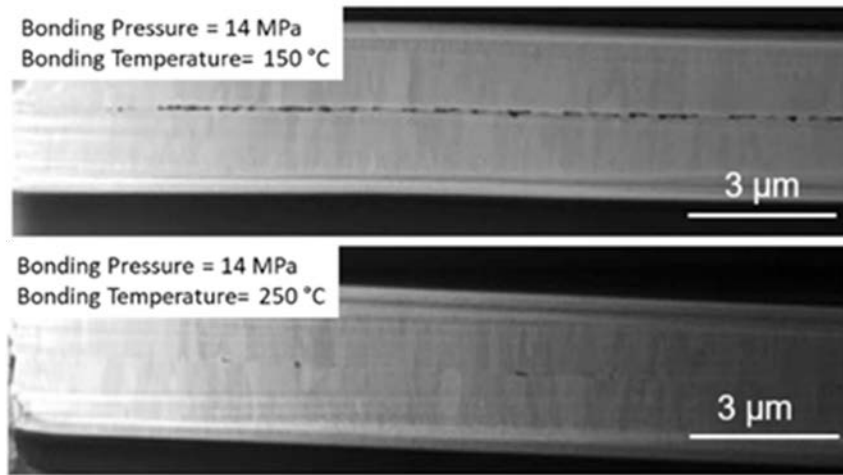
Fig 3. SEM cross-section of bonded interfaces at different temperatures.
