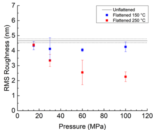
Fig 4. Roughness values before and after flattening at 150 and 250 °C (dotted lines are the standard deviation for unflattened sample)
