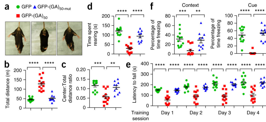
Figure 7. Poly(GA) mice develop motor deficits, hyperactivity, anxiety and cognitive defects. (a) Response of mice expressing GFP, GFP-(GA) 50 or GFP-(GA) 50-mut after tail suspension. Splayed hind legs are indicative of a normal escape response. (b–d) Results from the open field test analyzing the behavior of mice expressing GFP, GFP-(GA) 50 or GFP-(GA) 50-mut ( n = 10–12 per group), where hyperactivity is indicated by the total distance traveled (b) , signs of anxiety are manifested by a decrease in the ratio of distance traveled in the center area to total distance traveled (c) , and potential deficits in motor coordination are indicated by a decrease in rearing assessed using raised photobeams (d) . (e) Results from a four day rotarod performance test used to determine motor deficits of mice expressing GFP, GFP-(GA) 50 and GFP-(GA) 50-mut ( n = 10–12 per group) by evaluating latency to fall from a rotating rod. (f) In the fear conditioning test, associative learning and memory of mice expressing GFP, GFP-(GA) 50 or GFP-(GA) 50-mut ( n = 10–12 per group) were evaluated by the percent of time freezing in response to an unconditioned (context) or conditioned (cued) stimulus. Data are presented as mean \pm s.e.m. In b , d and e : P < 0.0001 , one-way ANOVA; **** P < 0.0001 , Tukey's post hoc analysis. In c : P = 0.0001 , one-way ANOVA; *** P = 0.0002 and ** P = 0.0022 , Tukey's post hoc analysis. In f (left): P = 0.0005 , one-way ANOVA; *** P = 0.0009 and ** P = 0.0042 , as assessed by Tukey's post hoc analysis. In f (right): P < 0.0001 , one-way ANOVA; **** P < 0.0001 , Tukey's post hoc analysis.
