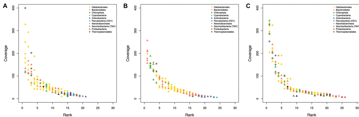
FIGURE 3 | Rank abundance curves from ribosomal protein S3 coverage from the assembled metagenomic reads at the (A) wettest site, (B) intermediate site, (C) and driest site.
