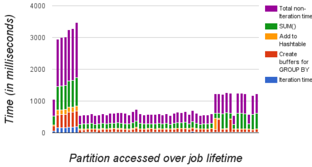
Figure 5: Code generation optimizes memory access rates for Query 2
