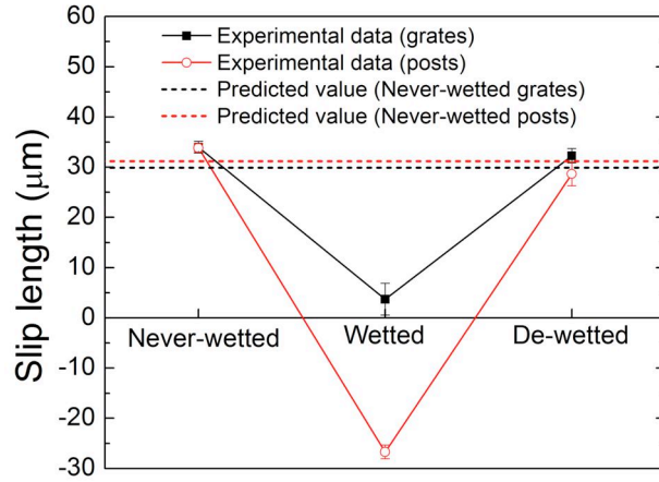
FIG. 4. Slip measurements with intentional wetting and active de-wetting underwater. Samples are a grid array of microposts (50 μm pitch, 90% gas fraction) and a concentric array of microgrates (80 μm pitch, 80% gas fraction), tested in succession: never-wetted (voltage on), wetted (voltage off), and de-wetted (voltage on). Each error bar represents the standard deviation of five data points.
