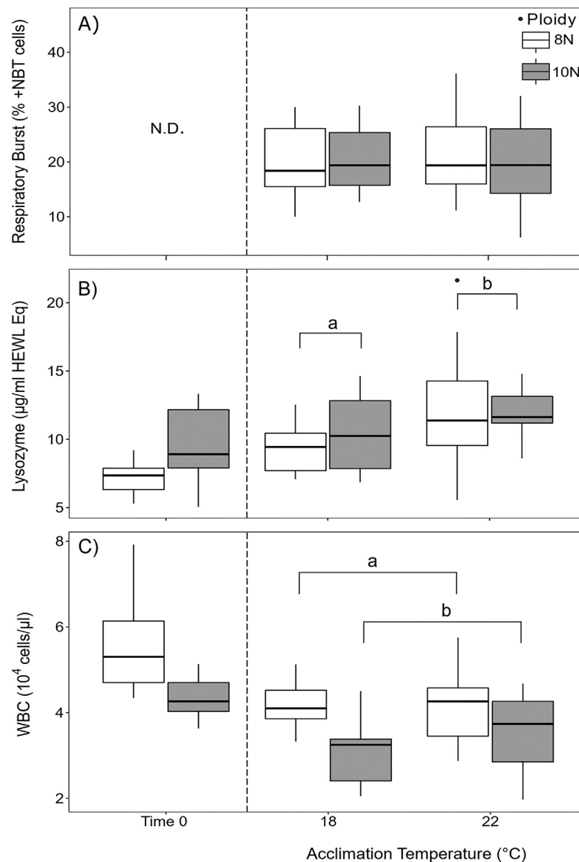
Fig. 2. Respiratory burst activities (A), plasma lysozyme (B) and total leukocyte counts (C) of 8 N and 10 N white sturgeon before (Time 0, n = 6) and after a 6-week temperature acclimation (n = 12). Different letters denote significant differences between temperature or ploidies after temperature acclimation ( p < 0.05 ). An asterisk (*) denotes significant differences between ploidies at Time 0 ( p < 0.05 ). N.D. = not determined, NBT = nitro blue tetrazolium.
