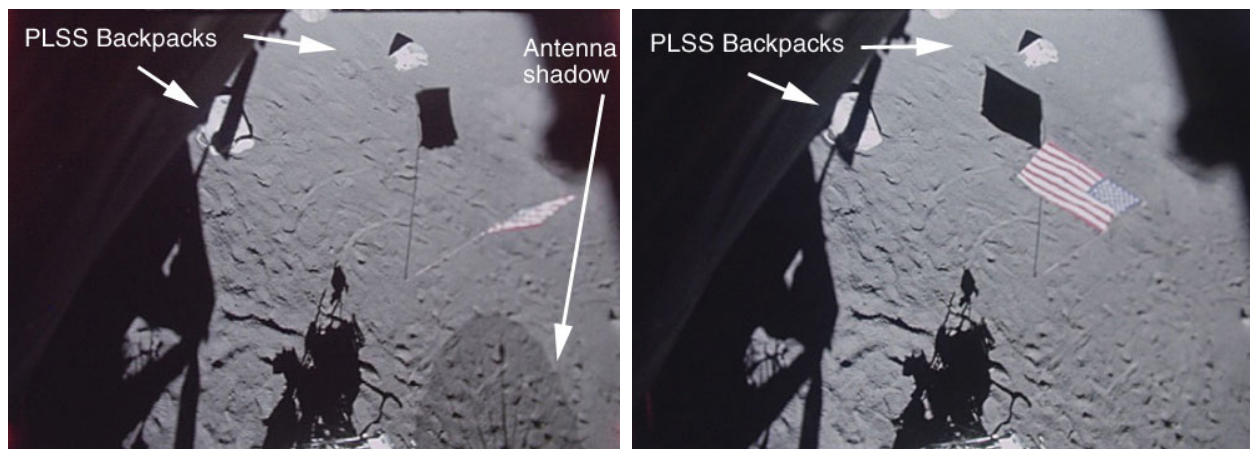
Figures 19–20: Two “smoking gun” images extracted from Apollo 14 video footage by Robert Godwin. Notice that in the photo at left the fly of the flag goes to the right, and in the one at right the fly is going to the left. There are no astronauts in the transitional frames who could have moved the flag, so what has happened? Conspiracy theorists claim that flag movement in moon landing videos was caused by the wind, but there is a more rational explanation—the flag was flipped by the force of testing the engines on the lunar module. (Photos extracted and labeled by Robert Godwin).
