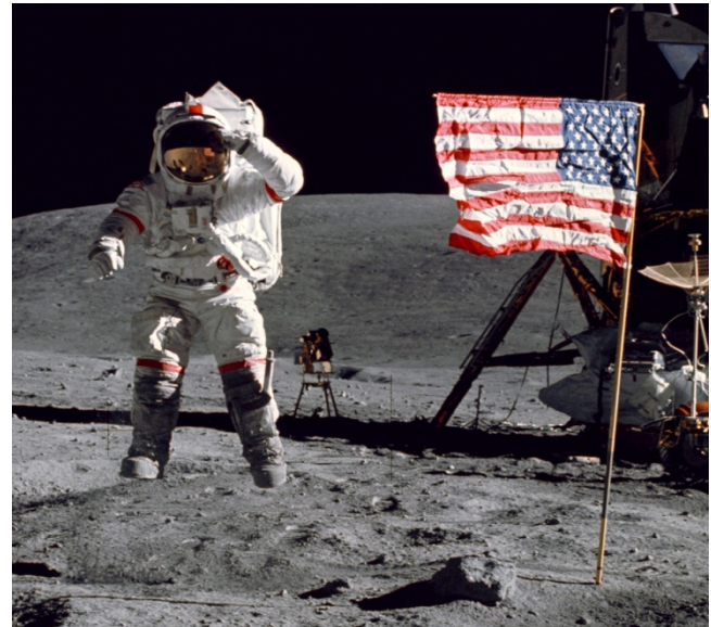
Figures 16–18: Extract from an Apollo 16 video showing astronaut John Young’s famous jump salute from behind (top). Compare this view to the still photo of the event taken from the other side of the flag (bottom left) and an extract of that same image flipped horizontally and enlarged (bottom right). NASA Photograph AS16-113-18339 (21 April 1972).
