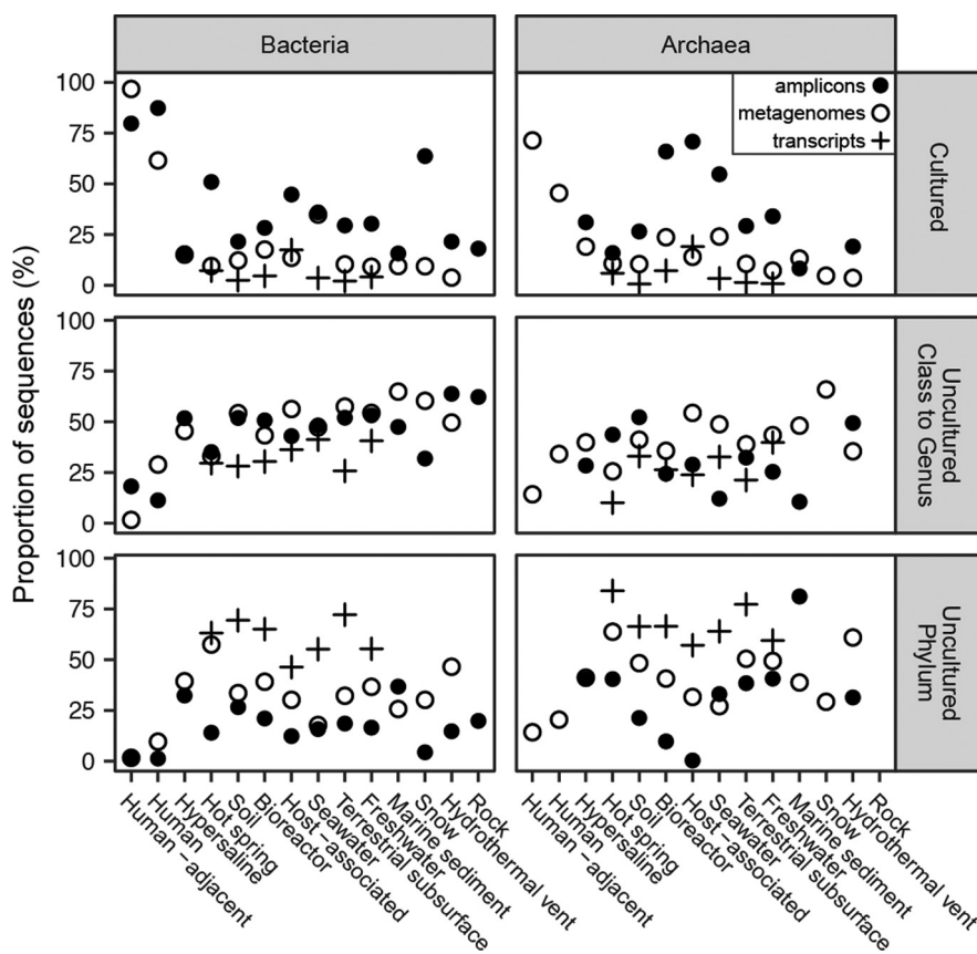
FIG 2 Proportion of 16S rRNA gene sequences in each category of phylogenetic novelty relative to cultures for each environment, by amplicons, metagenomes (without scaffold read depth), and metatranscriptomes. Closed circles represent primer-amplified amplicons, open circles represent metagenomes, and crosses represent transcriptomes. Total numbers of sequences and studies are listed in Table S2.
