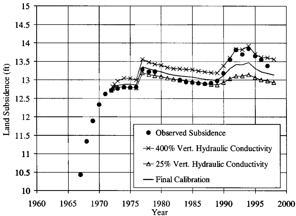
Figure 31(f) - Extensometer 6
