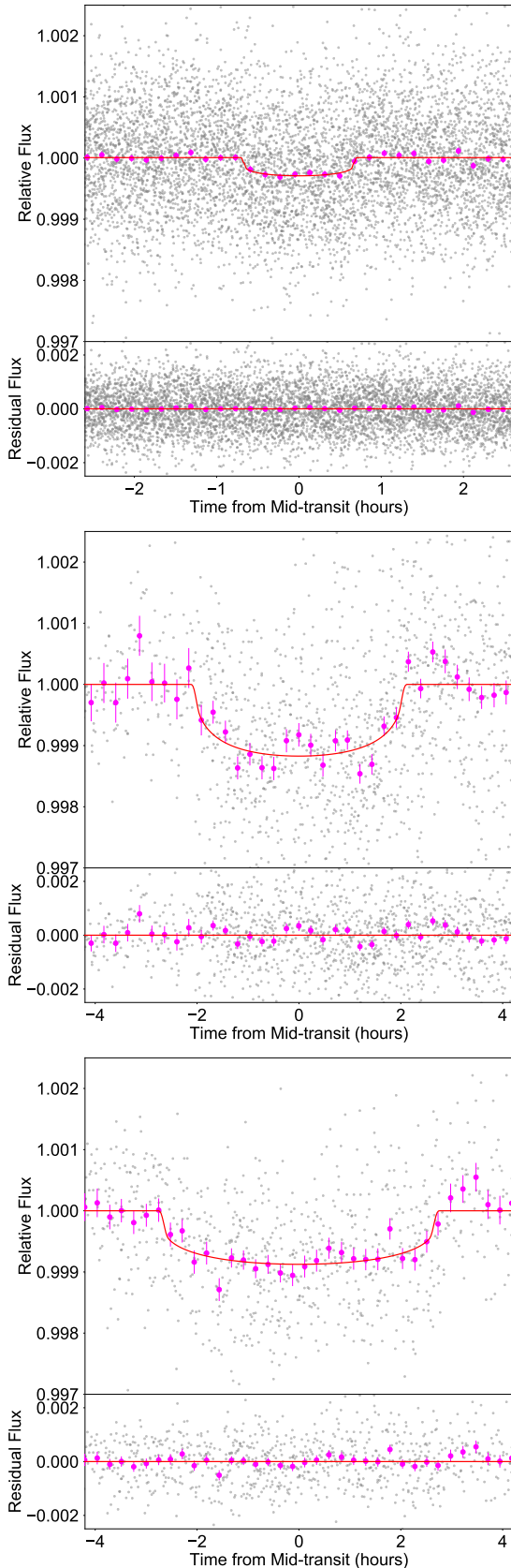
Figure 6. The phase-folded transits of TOI-561 planets b (top), c (middle), and d (bottom). We removed regions where two planets transit simultaneously before plotting. The magenta points show binned fluxes. The red solid line shows the best-fit transit models.
