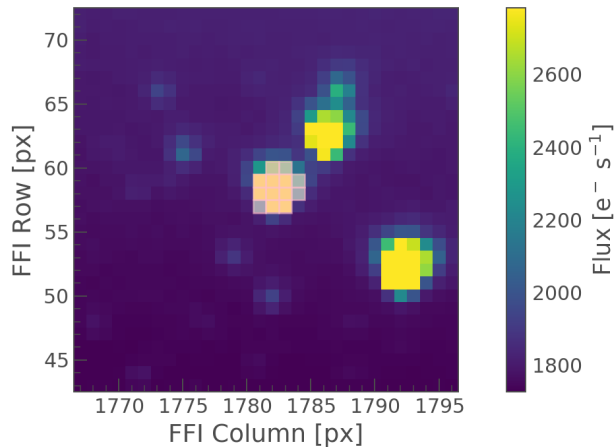
Figure 2. The TESS Full-Frame Image centered on TOI-561. The SPOC-defined aperture is a pale pink overlay on the central star. The TESS plate scale is 21'' per pixel. The target star has TESS magnitude 9.49. False positive scenarios in which the bright nearby stars are eclipsing binaries, with some flux contaminating the target pixels, are ruled out with the data validation centroid test (planet d) and/or follow-up ground based photometry (§4, planets b and c).
