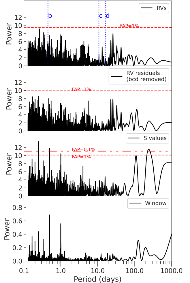
Figure 9. Lomb-Scargle periodograms of (a) the RVs, (b) the RVs after removing the best-fit [Model B] RV signatures from planets b, c, and d, (c) the Mt. Wilson S-value stellar activity indicator time series, and (d) the window function. False alarm probabilities (FAPs) are computed based on a bootstrap resampling of each time series. The RVs and RV residuals do not have any peaks that cross the 1% FAP. The S-values have significant ( \text{FAP} > 1\% ) peaks at 100 days, 230 days, and various short periods that are likely aliases of the longer-period signals caused by the window function.
