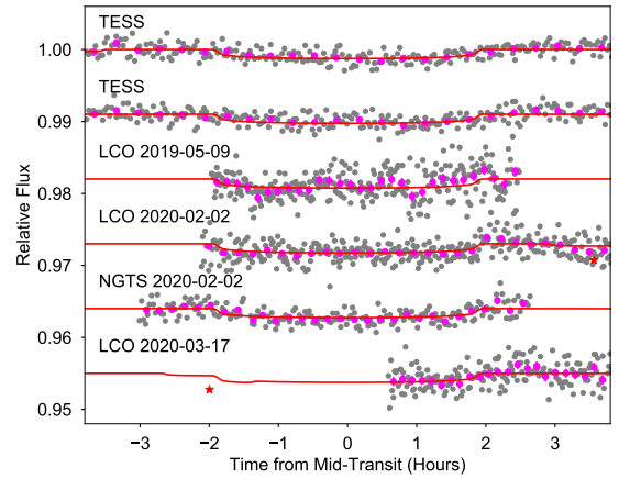
Figure 5. The individual transits of planet c from TESS and ground-based facilities. The magenta points are binned data. The red stars indicate the mid-transits of planet b which due to the short orbital period often overlap with the transits of planet c and d. The red solid is the best fit global model that include both TESS and ground-based photometry and model transits of all three planets simultaneously. Note that the ground-based transits of planet d were acquired at times that are not consistent with our best-fit ephemeris, and they are not shown.
