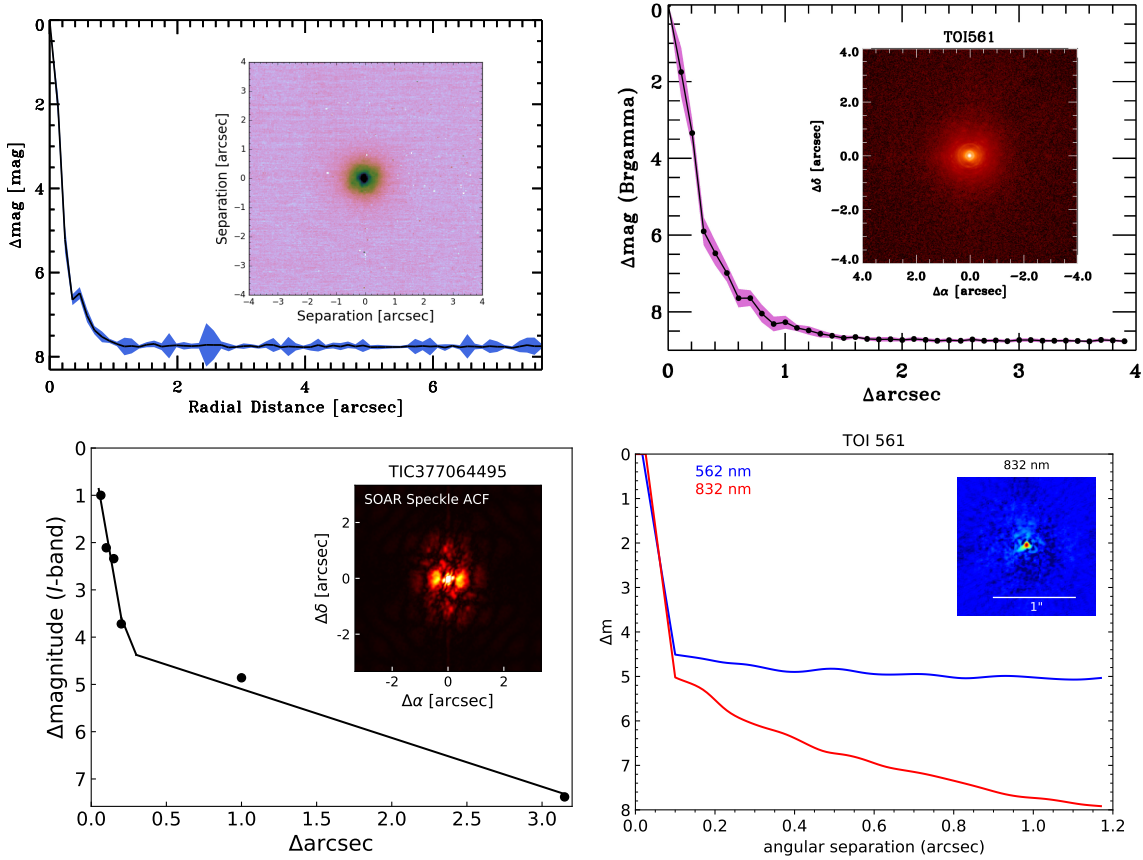
Figure 7. No nearby stars were detected in 4 independent imaging campaigns. Top left: Sensitivity to background stars of our Gemini-N/NIRI images in the Br \gamma filter. The images were taken in good seeing conditions, and we reach a contrast of 7.5 magnitudes fainter than the host star within 0.''5. Inset: Image of the central portion of the data, centered on the star. Top right: Same as top left, but with Palomar. Bottom left: sensitivity to background stars from SOAR speckle imaging observations (5- \sigma upper limits), with an example image inset. Bottom right: Same as bottom left, but with Gemini-S/Zorro in two passbands.
