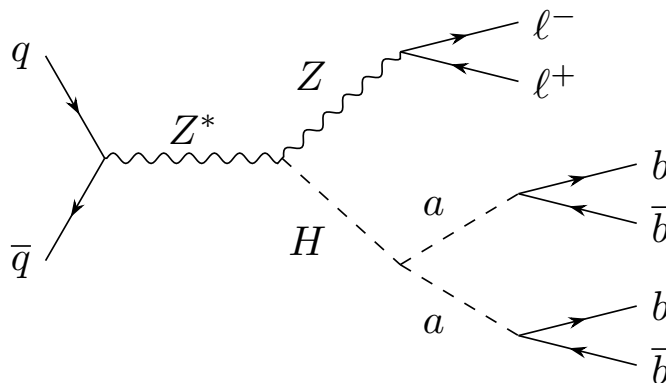
Figure 1. Tree-level Feynman diagram representing ZH production with H \rightarrow aa \rightarrow \bar{b}b\bar{b}b .
