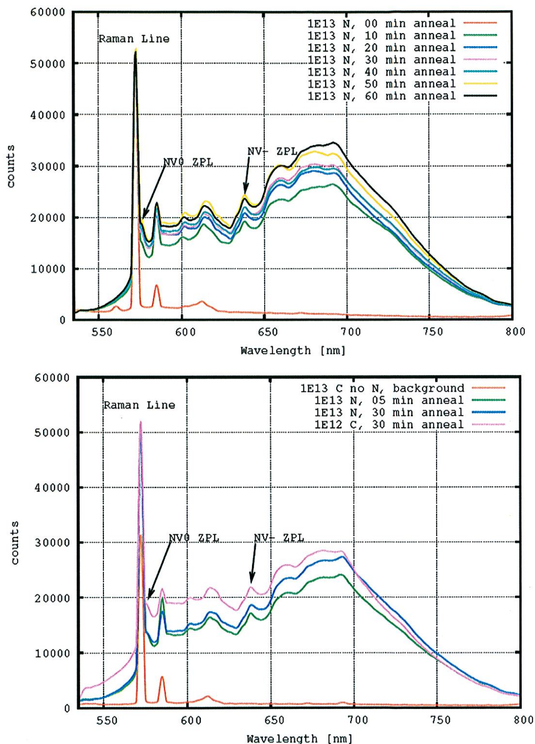
Figure 2: Examples of PL spectra (room temperature) from diamond samples following implantation of a) nitrogen ions ( 10^{13}\text{ cm}^{-2} ) and for a series of annealing times, b) for N-implantation and co-implantation of carbon ions with the sample at 780^\circ\text{C} during implantation ( 10^{12}\text{ cm}^{-2} , implant time 10 min.) and for a series of annealing times. The red curve in b) shows the background spectrum from C-implantation only, without prior N-implantation.
