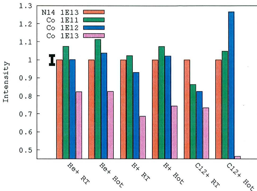
Figure 4: Histogram summarizing NV-PL intensity evolution for co-implantation of helium, hydrogen and carbon ions (all 7.7 keV, normal incidence) into diamond samples held at room temperature or heated to 780°C during implantation. A representative error bar is shown for the N-only implant in the He co-implantation at room temperature series.
