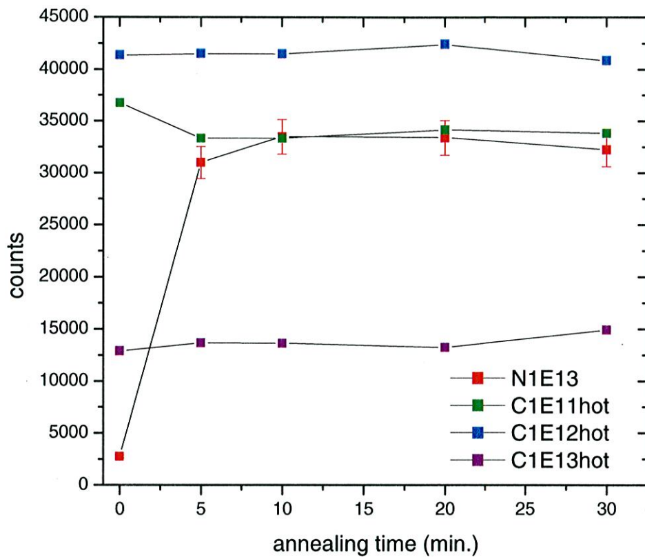
Figure 4: PL intensities from NV-centers ( \text{NV}^- and \text{NV}^0 ) as a function of annealing time and for a series of co-implantation fluences for co-implantation with carbon ions (7.7 keV, normal incidence) and with diamonds heated to 780° C during co-implantation. Representative error bars are shown for the N-only implant series ( 10^{13} \text{ cm}^{-2} , 7.7 keV, normal incidence). Lines are drawn to guide the eyes.
