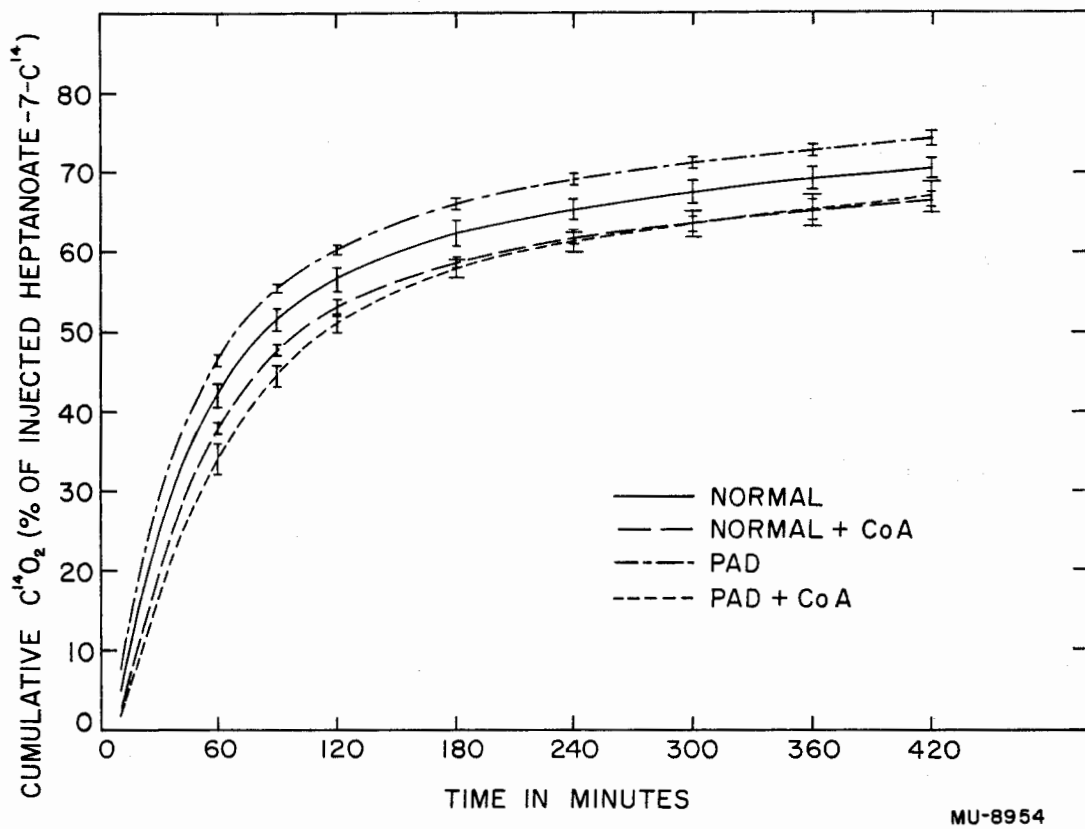
Fig. 12. Cumulative excretion of C^{14}O_2 in normal and PAD rats following administration of sodium heptanoate-7- C^{14} .
