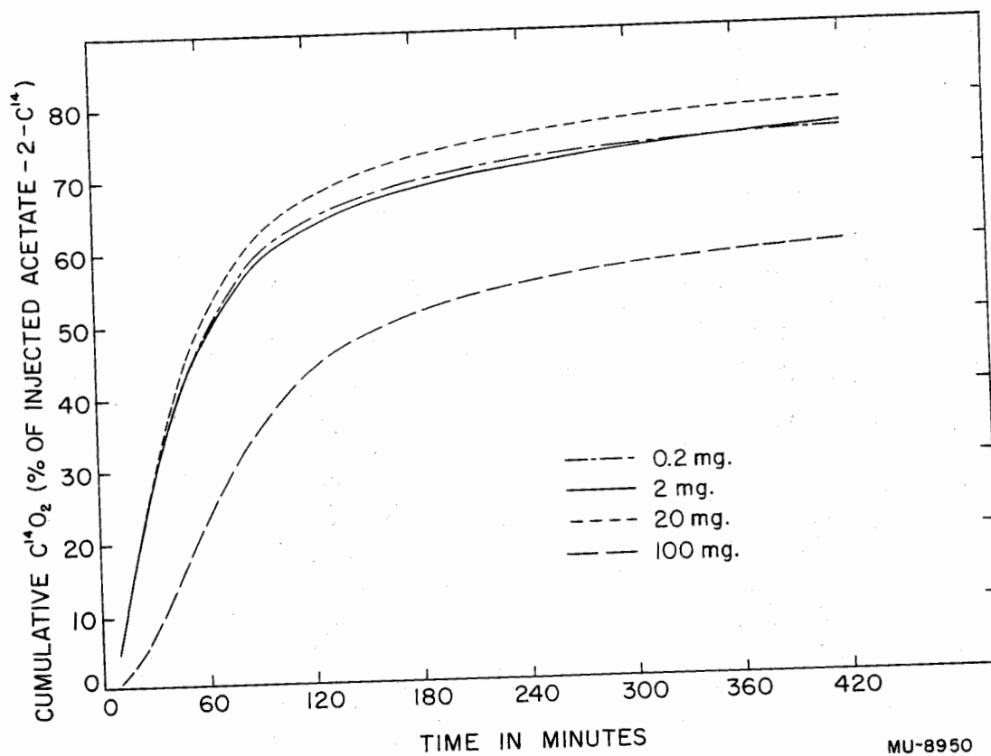
Fig. 8. Effect of substrate concentration on the cumulative excretion of C 14 O 2 following administration of sodium acetate-2-C 14 in normal rats.
