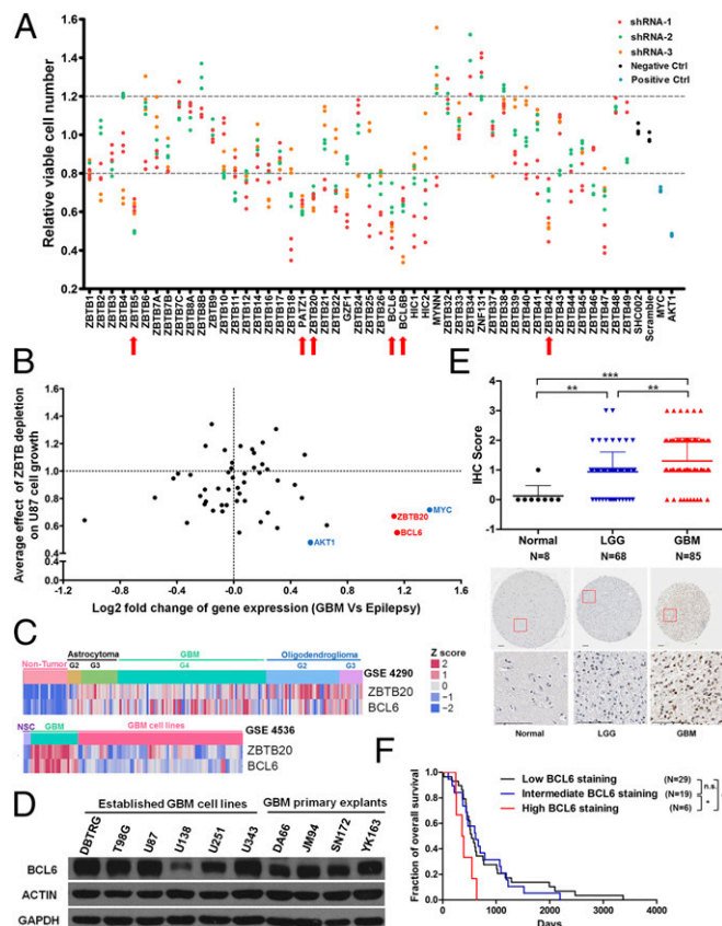
Fig. 1. Identification of BCL6 as a progrowth factor in glioma. ( A ) Relative viable number of U87 GBM cells after infection with lentiviral particles encoding indicated shRNAs. SHC002 and pLKO-scramble were used as negative controls (Negative Ctrl), and shRNAs targeting MYC and AKT1 were used as positive controls (Positive Ctrl). Candidate genes (marked by red arrows) were selected only if all independent shRNAs and all repeats showed consistent increase or decrease (>20%) in relative viable cell number compared with negative controls. ( B ) Plot showing the correlation between average effect of ZBTB depletion on U87 cell growth and differential gene expression (GBM vs. epilepsy; GSE4290). BCL6 and ZBTB20 were highlighted in red as candidates for growth-promoting genes. MYC and AKT1 were marked in blue as positive controls for oncogenes. ( C ) Heat map showing the expression of BCL6 and ZBTB20 in nontumor brain tissues (epilepsy), GBM cell lines, and primary GBM samples. G2, G3, and G4 denote World Health Organization grade II, III, and IV, respectively. NSC, neural stem cells. ( D ) Western blot result showing the endogenous BCL6 expression among 6 established GBM cell lines and 4 primary GBM explants. ( E ) IHC results and representative staining images showing BCL6 expression in normal brain, LGG (lower-grade glioma), and GBM samples. (Scale bars, 100 \mu m). IHC scores were compared using a nonparametric statistical test. ( F ) Survival curves for patients with GBM with differential BCL6 expression (Low, IHC score 0 or 1; Intermediate, IHC score 2; High, IHC score 3). Log-rank test was applied.
