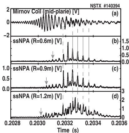
FIG. 5. Time traces of ssNPA measurements during a strongly chirping EPM mode on NSTX, for different tangency radii R = 0.6, 0.9, and 1.2 m. The signal from a Mirnov coil (top) provides a reference for the phase of the magnetic perturbation.
