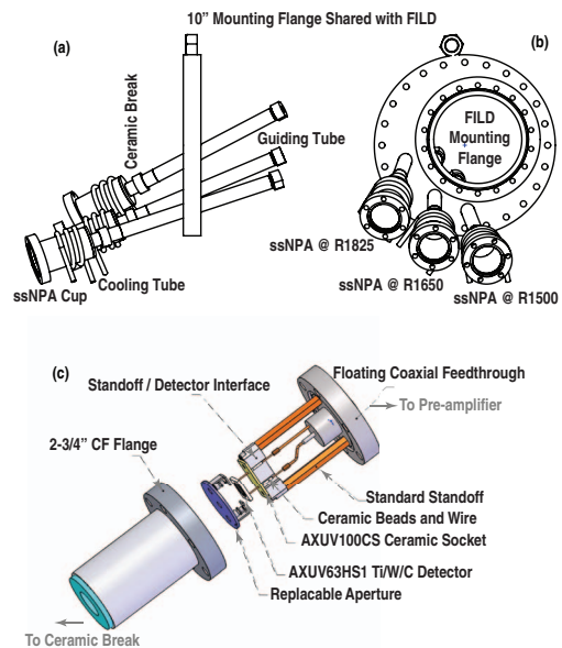
FIG. 2. CAD drawing for three-channel DIII-D ssNPA system. (a)–(b) geometric arrangement (c) ssNPA detector head assembly.
