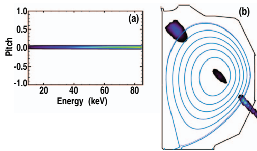
FIG. 1. The current mode ssNPA diagnostics retains excellent pitch resolution. Weight function in (a) velocity space and (b) configuration-space.
