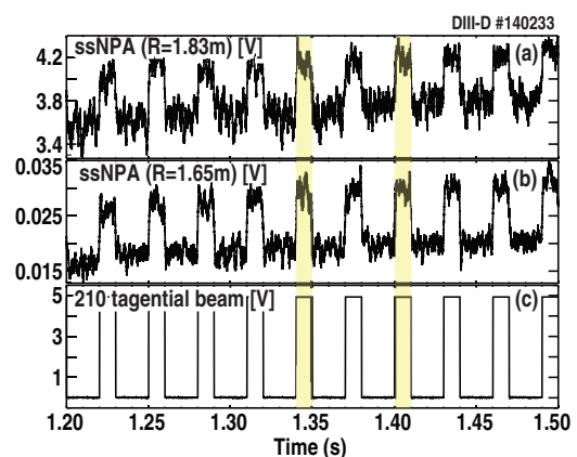
FIG. 3. DIII-D ssNPA system works in active CX mode.
