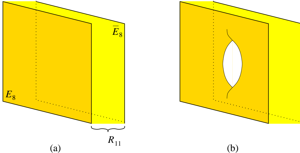
Figure 1: (a) A schematic picture of the E_8 \times \overline{E}_8 heterotic M-theory. The two boundaries are separated by distance R_{11} , carry opposite orientations, and support one copy of E_8 gauge symmetry each. (b) A schematic picture of the instanton responsible for the decay of spacetime to “nothing.” The instanton is a smooth throat connecting the two boundaries. Thus, the “bubble of nothing” is in fact a bubble of the hypothetical phase on the other side of the E_8 boundary.
