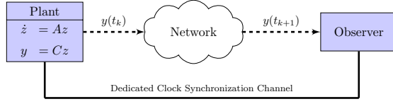
Figure 1.1: Block diagram of the networked plant-observer system.
