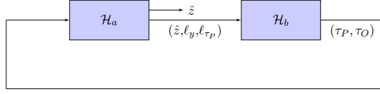
Figure 3.1: Diagram of the observer \mathcal{H}_a and clock synchronization \mathcal{H}_b subsystems and their interconnection.
