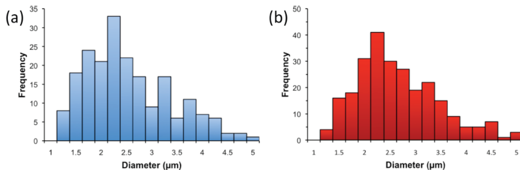
Figure 2.2: Size histograms for DSPC microbubbles made without (a) and with (b) added PAA from bright field microscopy. There were no bubbles larger than 5 \mu\text{m} found for either sample.
