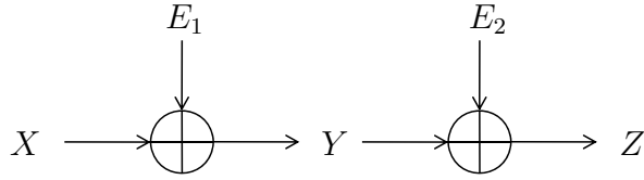
Figure 5.5: The physically degraded Gaussian wiretap channel.
