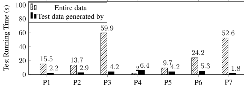
Figure 5.16: Test running time of entire data on large-scale cluster vs. testing on local machine with BIGTEST
